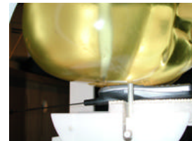
Fig. A Head SAR Test Setup
