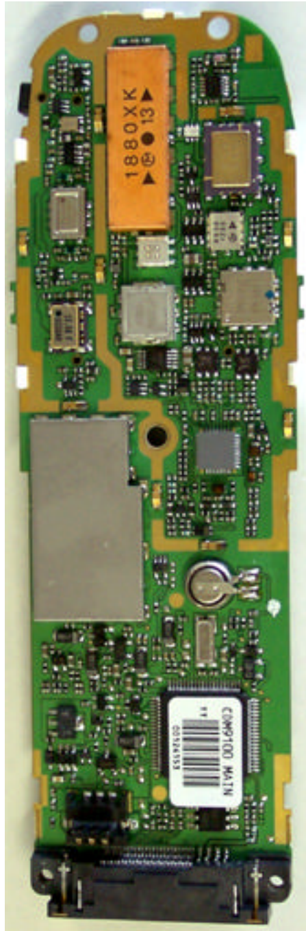
Handheld Portable MAIN Board (Back side , With shield cover removed) VCTCXO : VC-TCXO-204C2
