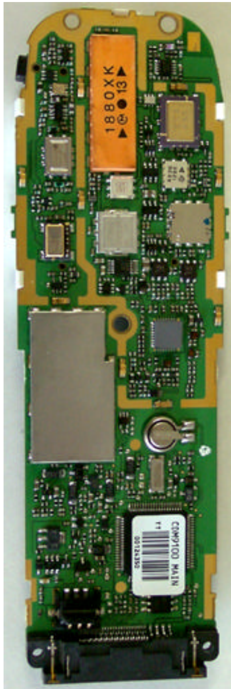
Handheld Portable MAIN Board (Back side , With shield cover removed) VCTCXO : DSA751HAD
