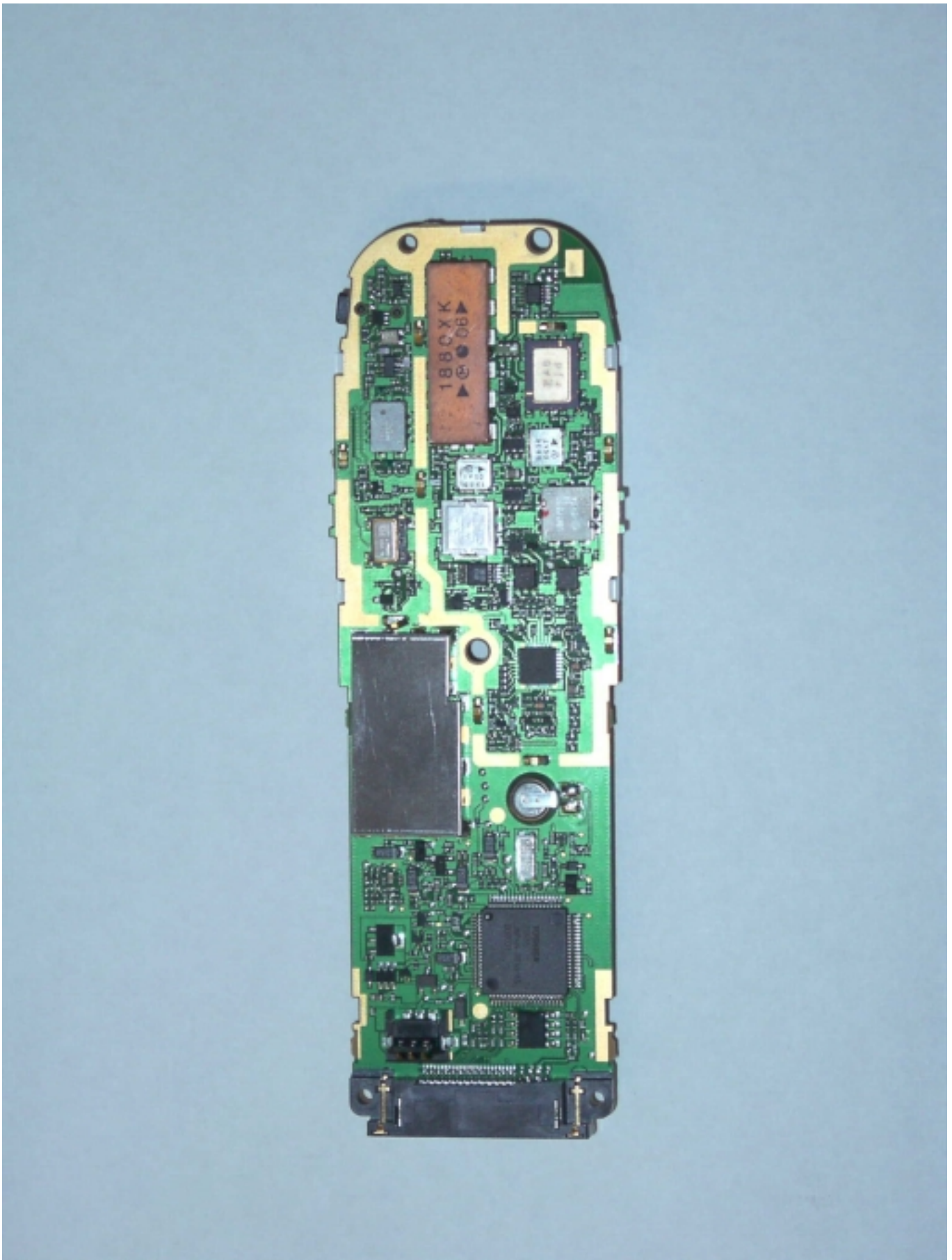
Handheld Portable MAIN Board (Back side , With shield cover removed)
