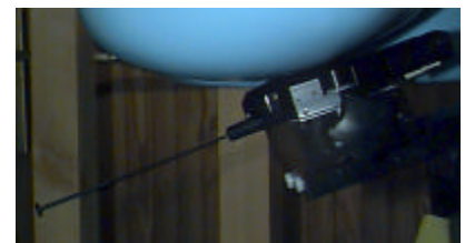
Figure 15. Head SAR Test Setup
