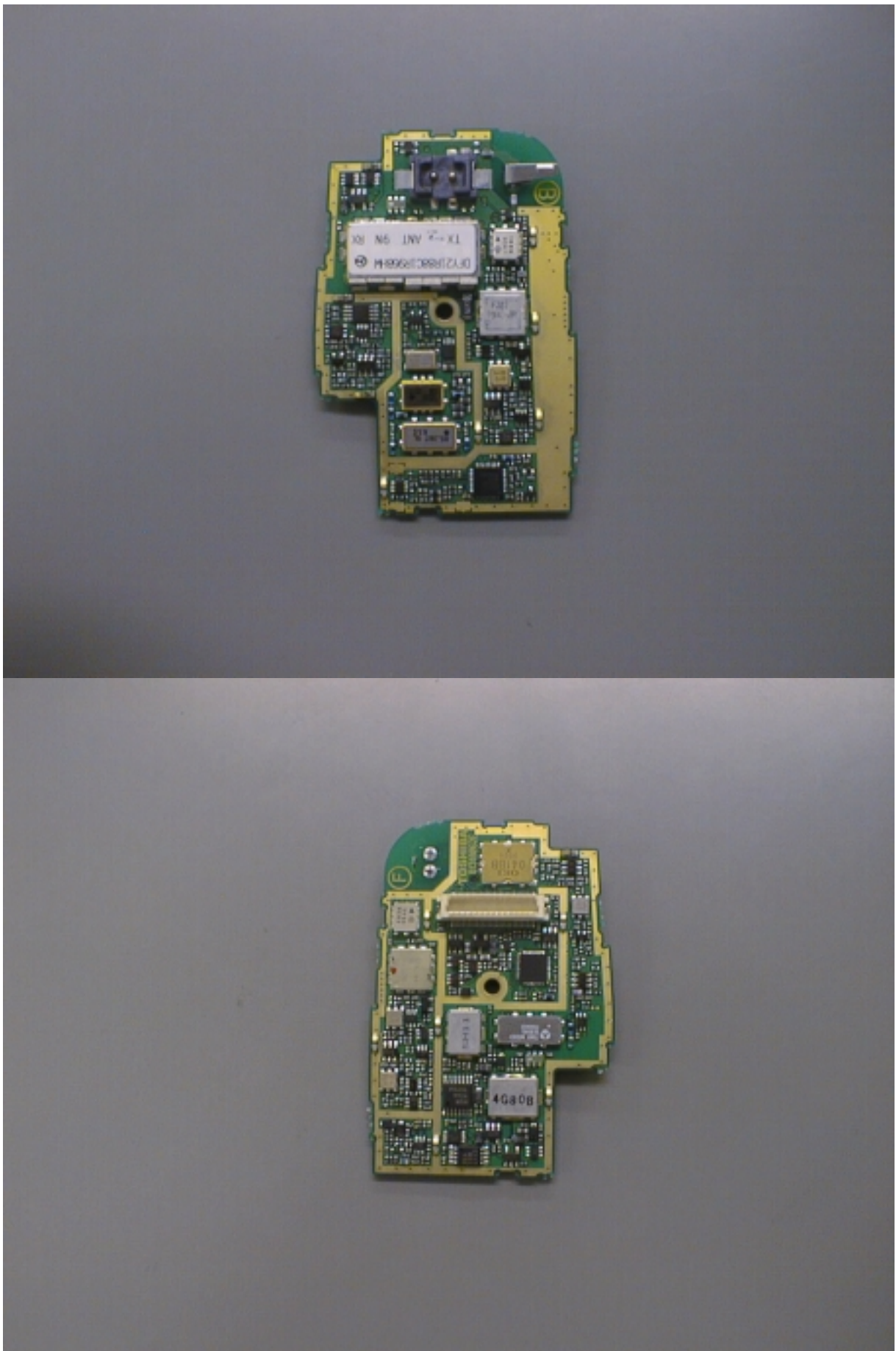
Handheld Portable TR Board (With Shelled Cover Removed)
