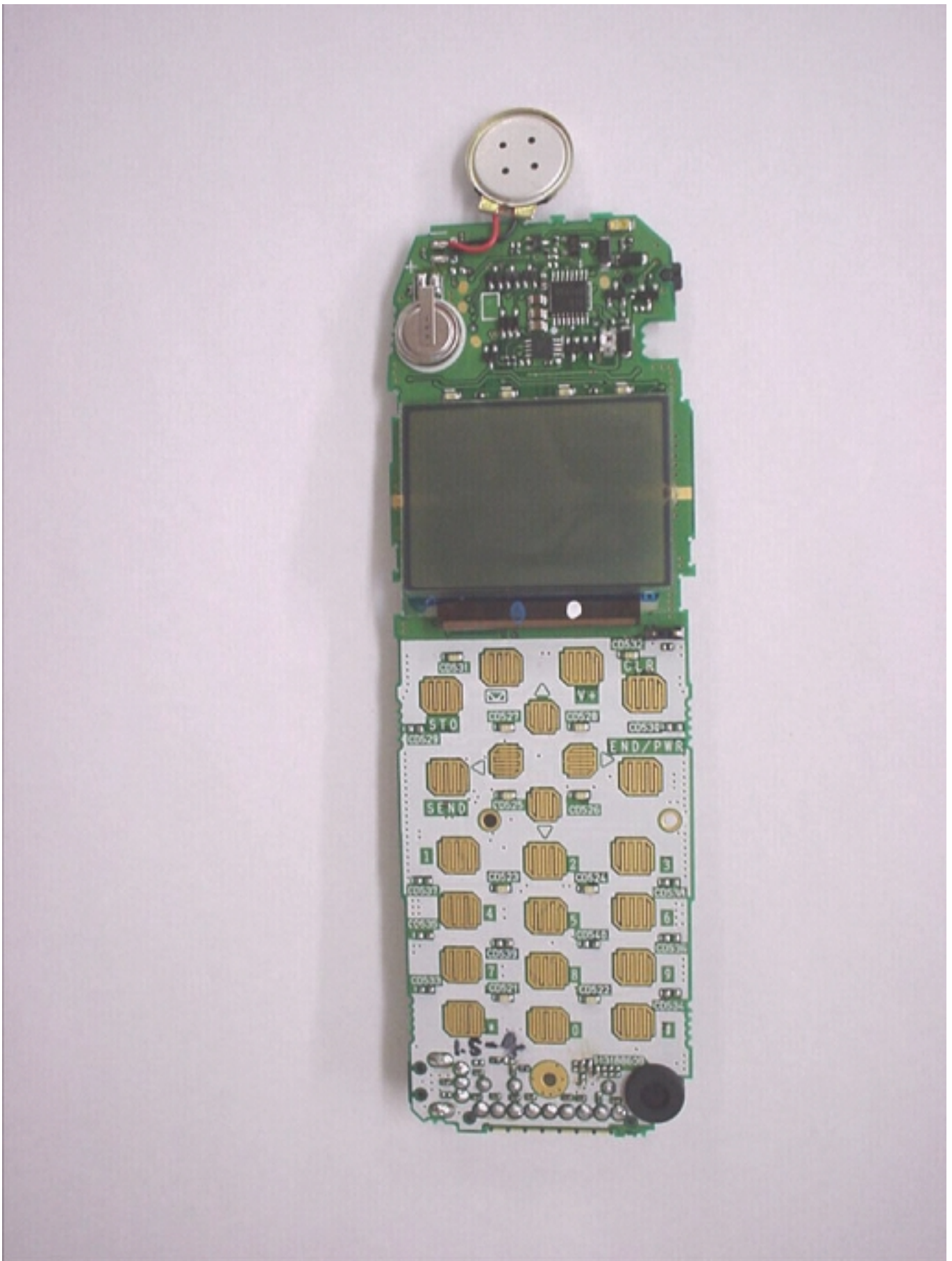
Handheld Portable CU Board (Front side)
