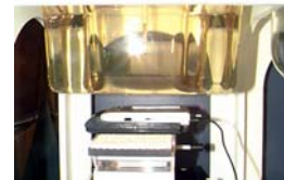
Figure 14.2 Face SAR Test Setup
