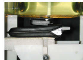
Fig. 16 Body SAR Test Setup
