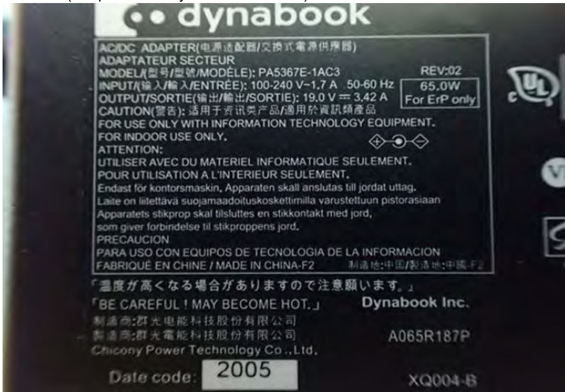
(15) EUT Photo (Adapter: Chicony / PA5367E-1AC3)
