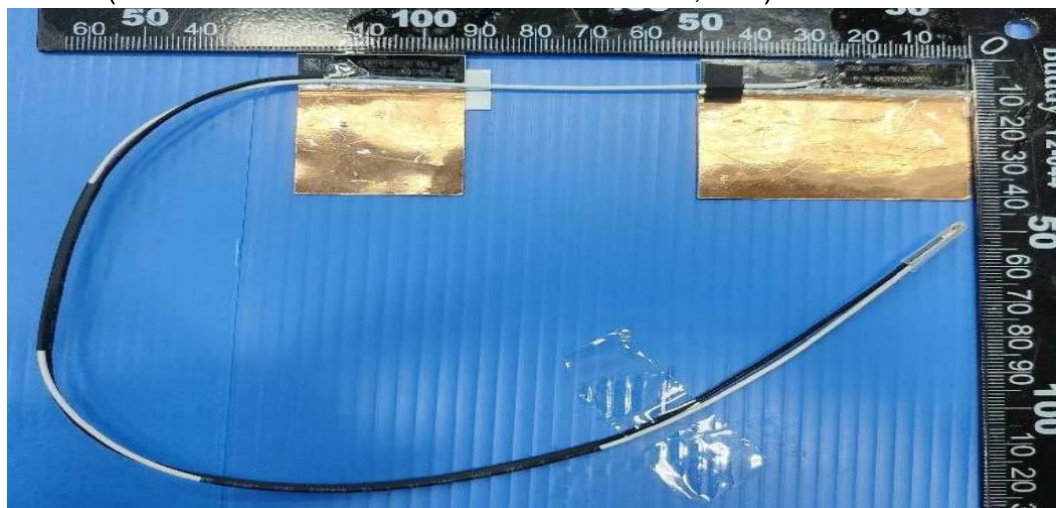
(28) EUT Photo (Antenna: SOUTHSTAR TECHNOLOGY CO.,LTD.)
