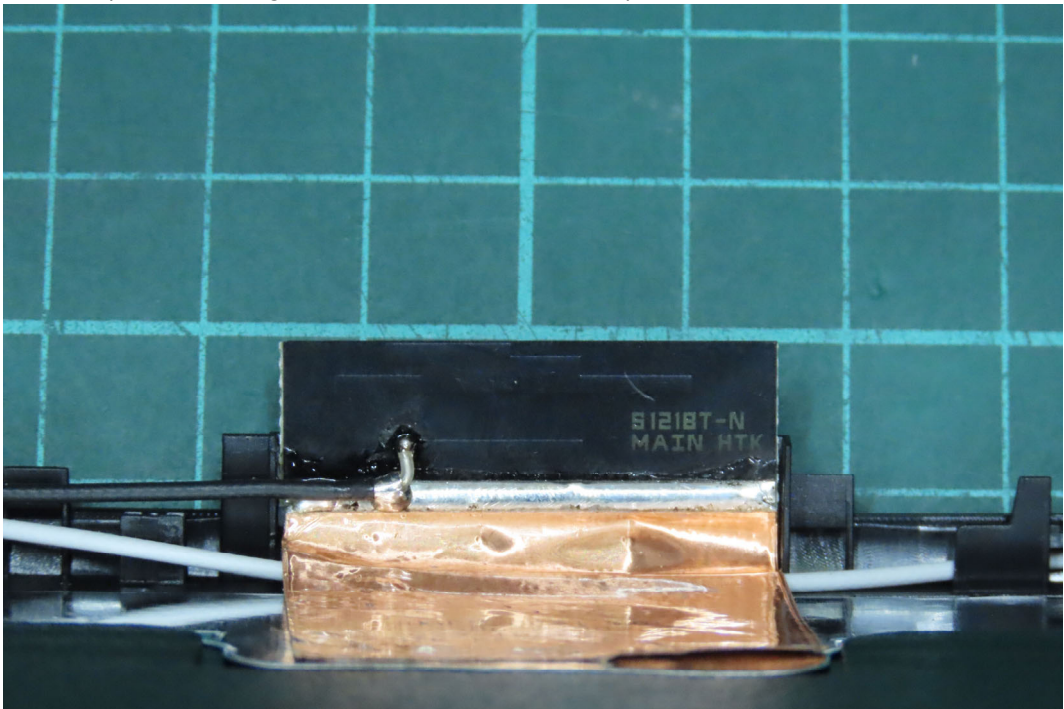
(26) EUT Photo (Antenna: High-Tek Electronics Co., Ltd.)
