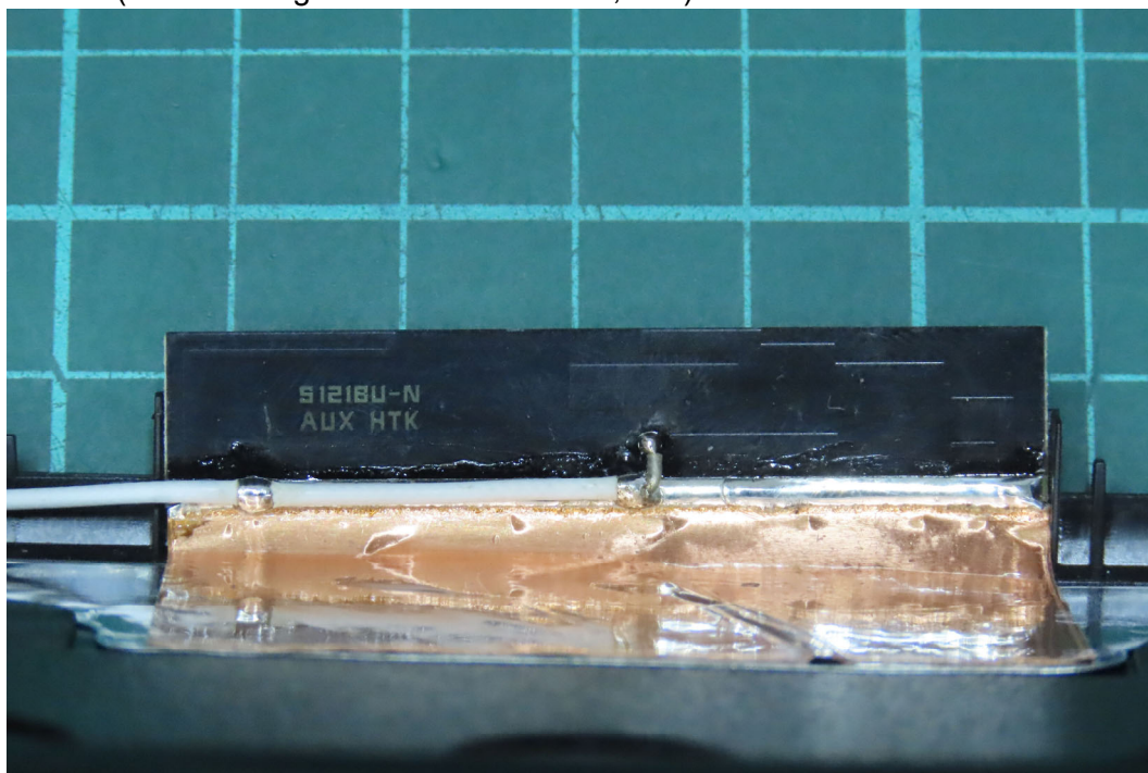
(27) EUT Photo (Antenna: High-Tek Electronics Co., Ltd.)
