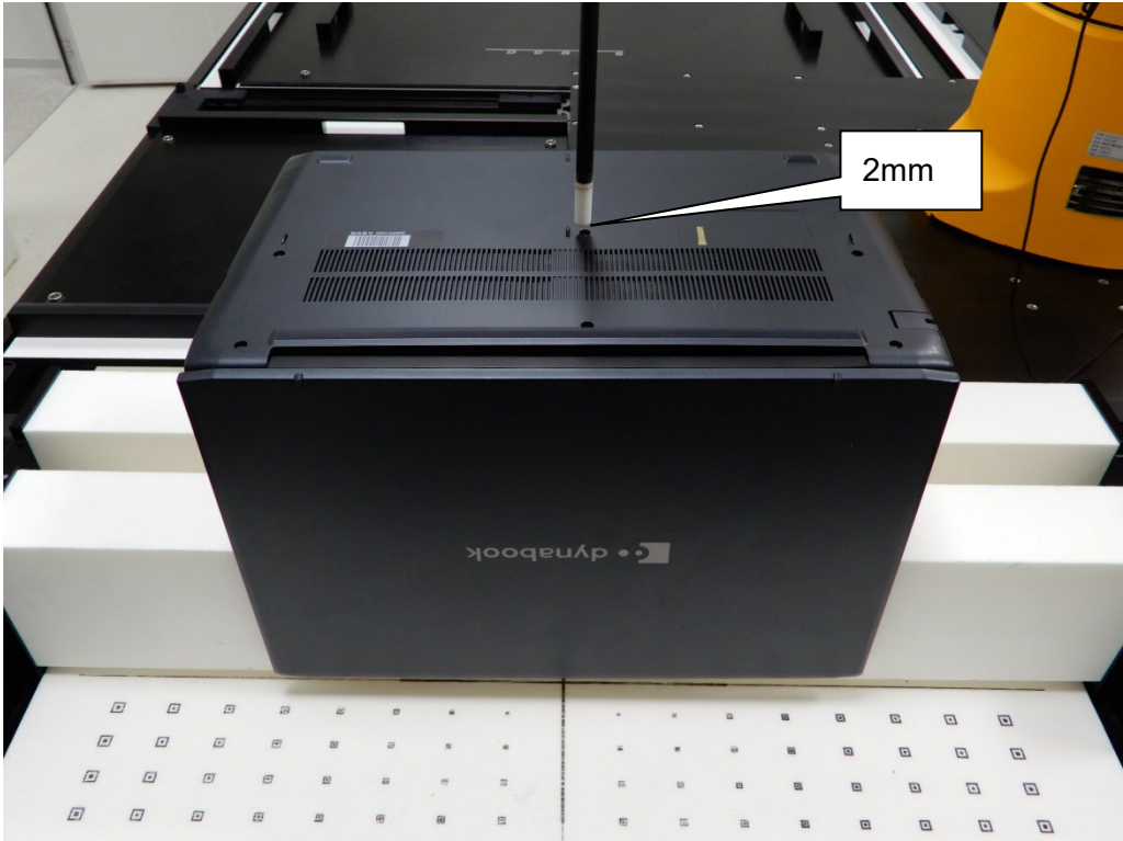
EUT Bottom_PD
