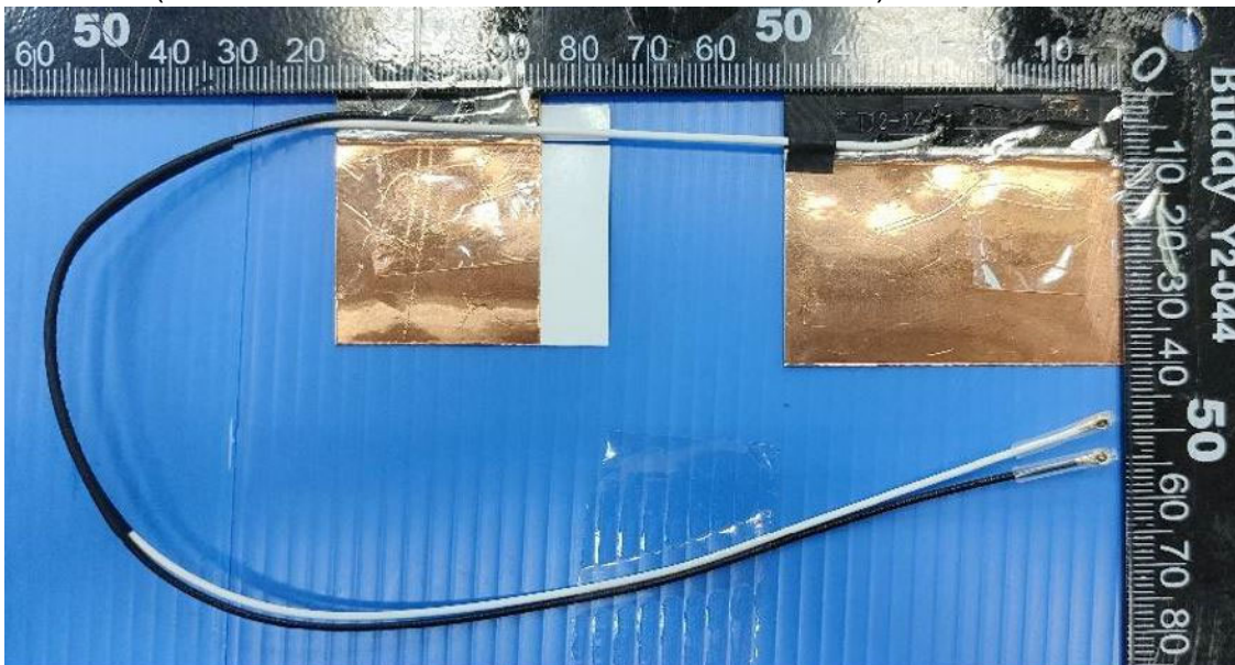
(72) EUT Photo (Antenna: SOUTHSTAR TECHNOLOGY CO.,LTD.)
