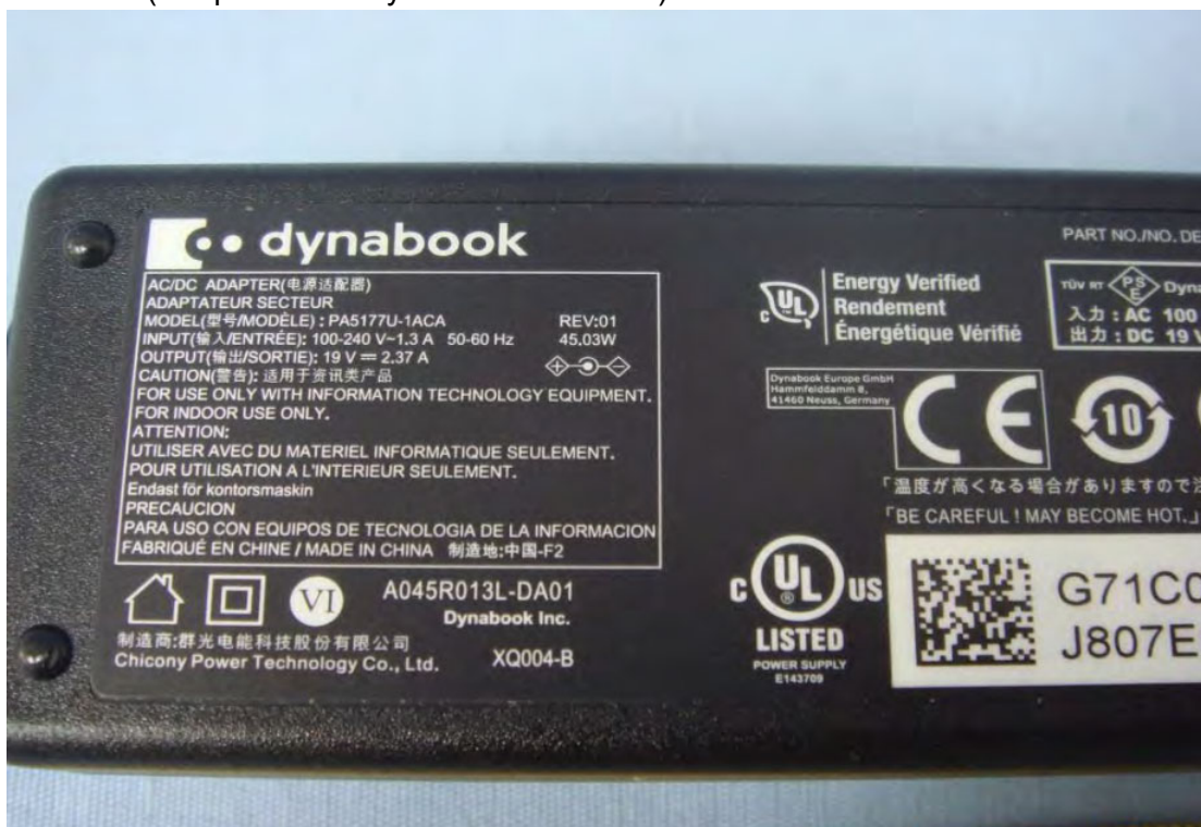
(23) EUT Photo (Adapter: Chicony / PA5177U-1ACA)
