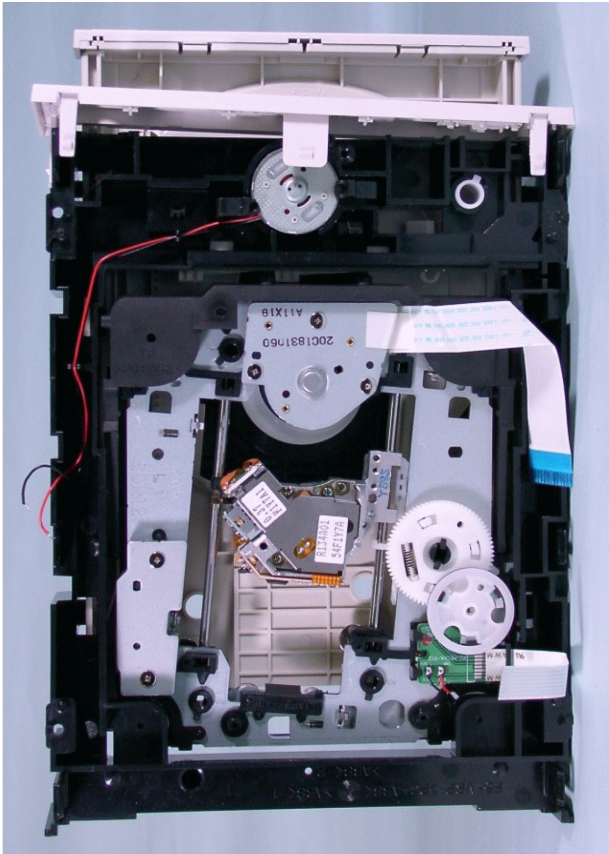
MECHANICAL Unit
