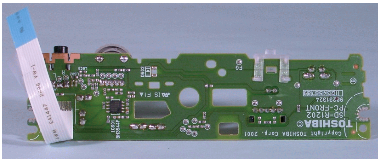
Front -PWB rear Location
