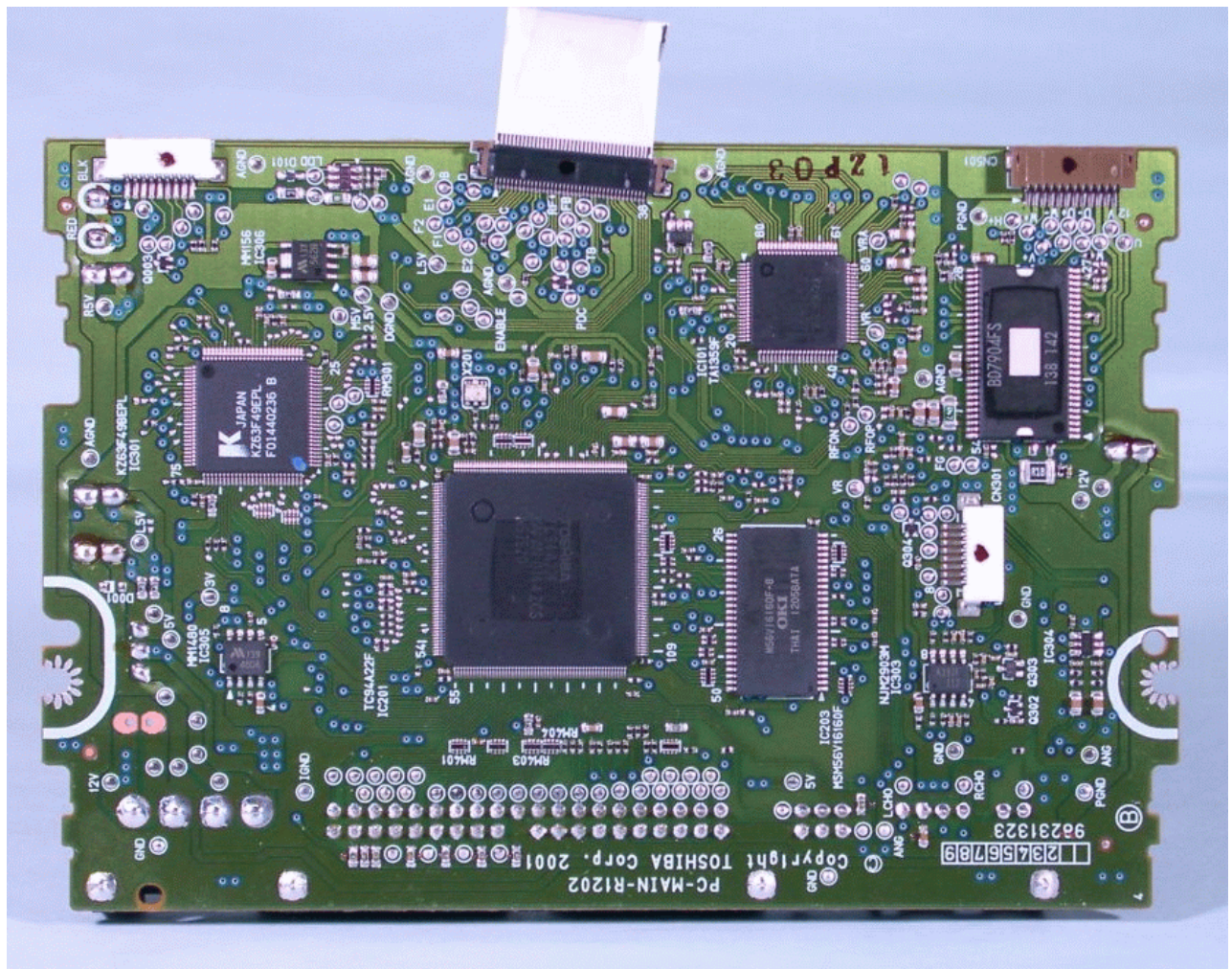
Main PWB rear Location
