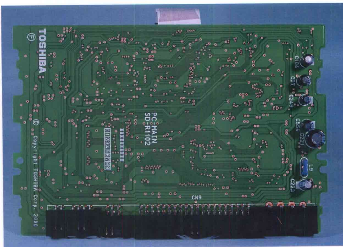
Main PWB Surface Location
