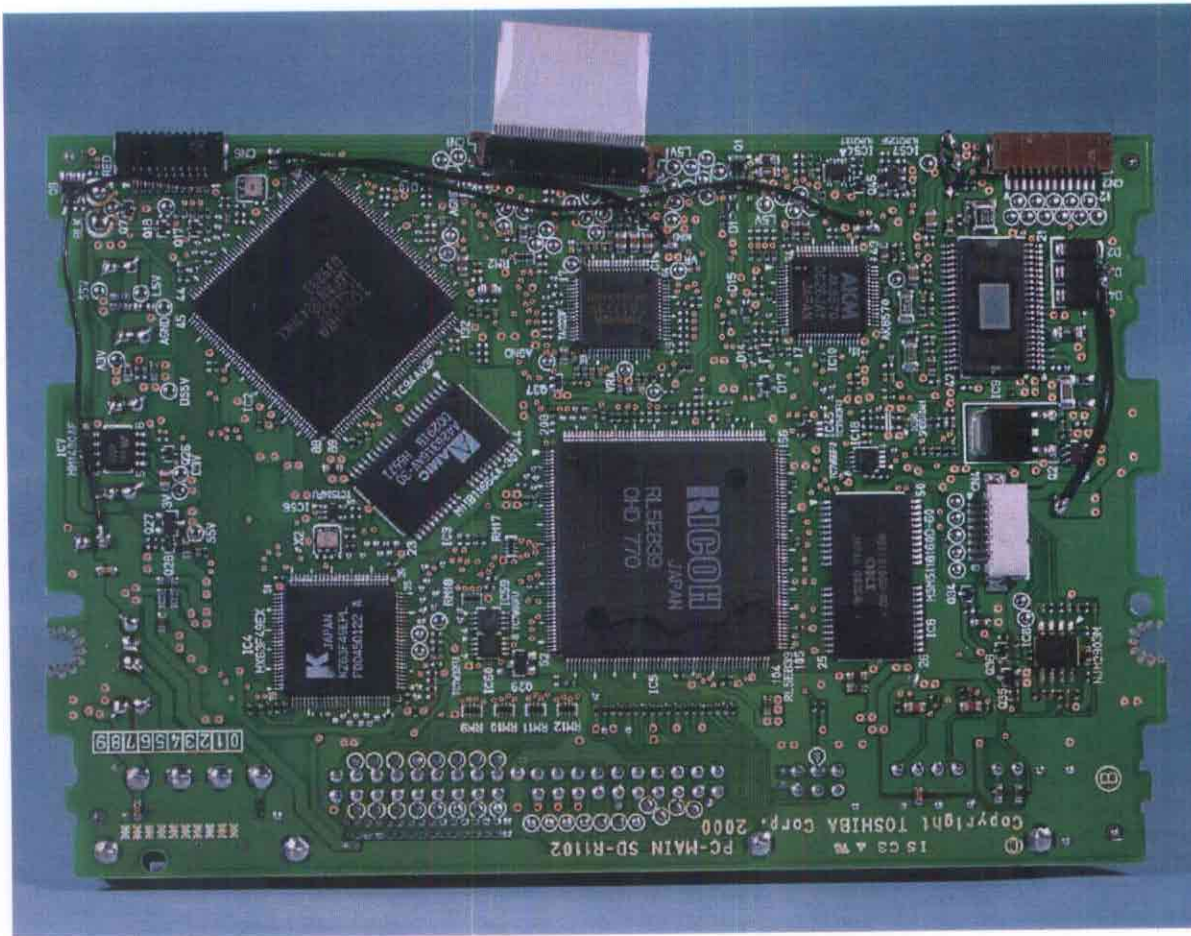
Main PWB rear Location
