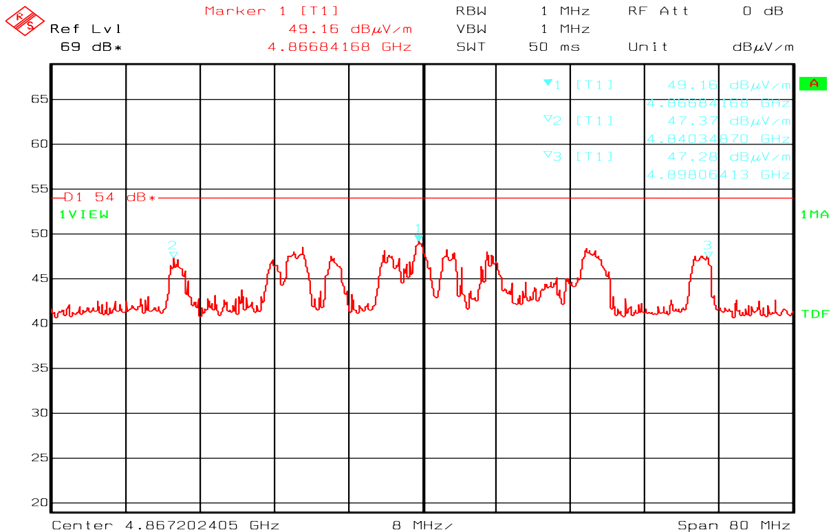
2 nd harmonic – Vertical Polarization
