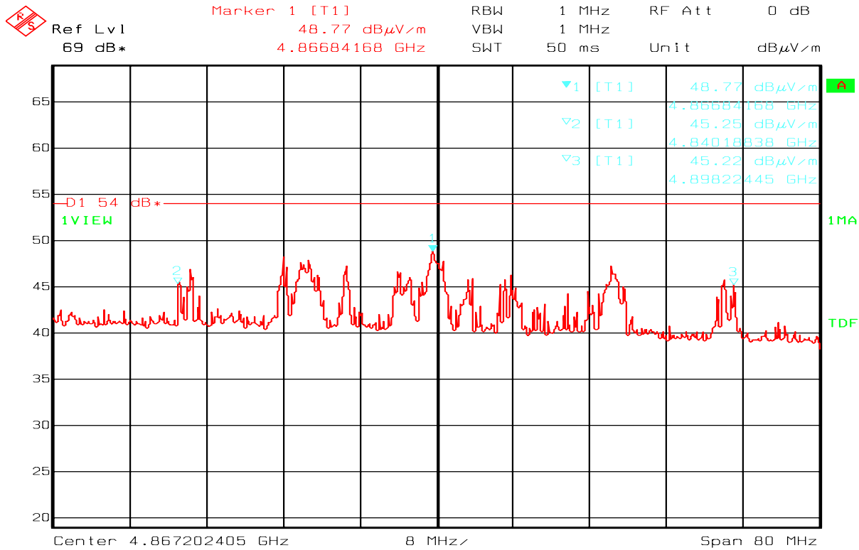
2 nd harmonic – Horizontal Polarization
