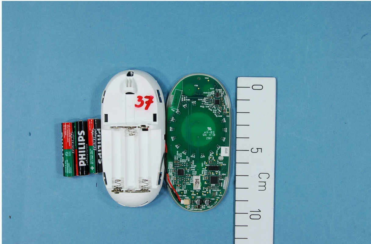
LC7 (Surf) – Remote control – Top view of PCB
