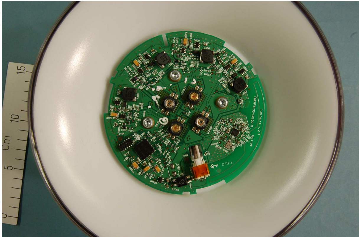
Luminaire – Top view of PCB
