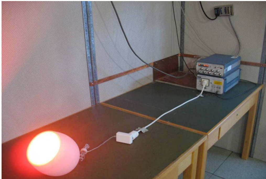
Photo 1: AC Line Conducted
