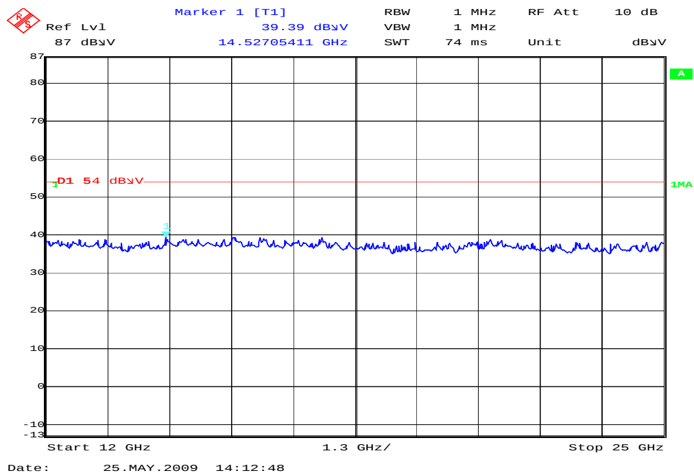
Plot 3: 12- 25 GHz (receiver)
