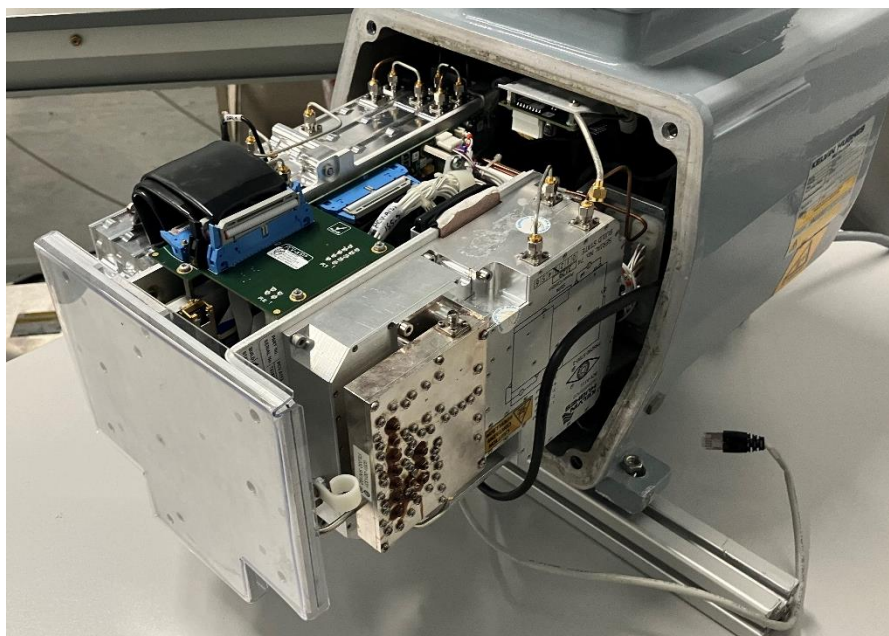
Internal of Mk5 Unit – SharpEye Assembly pulled out
