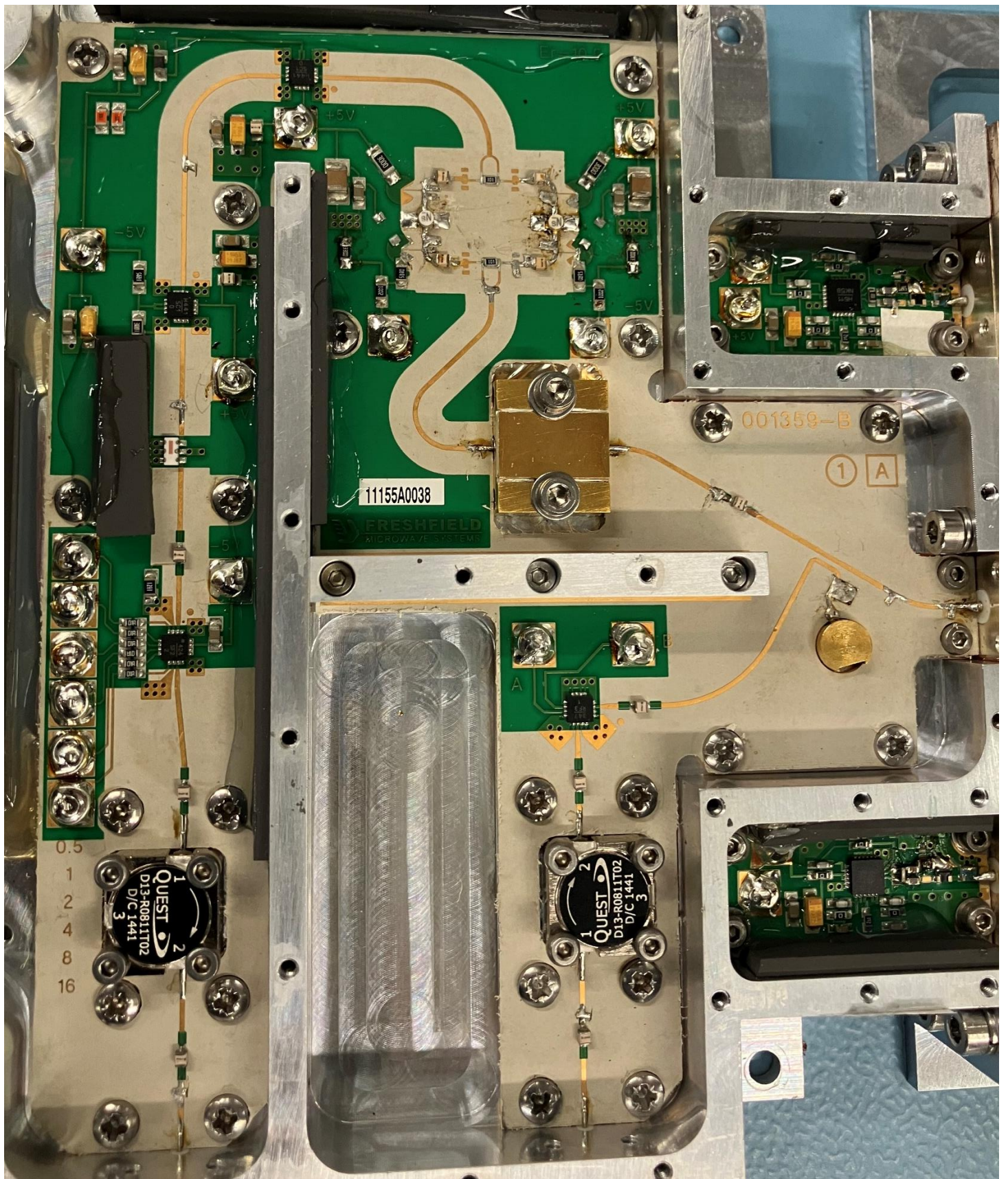
Internal – SCV LNA (PCB 001359-1)
