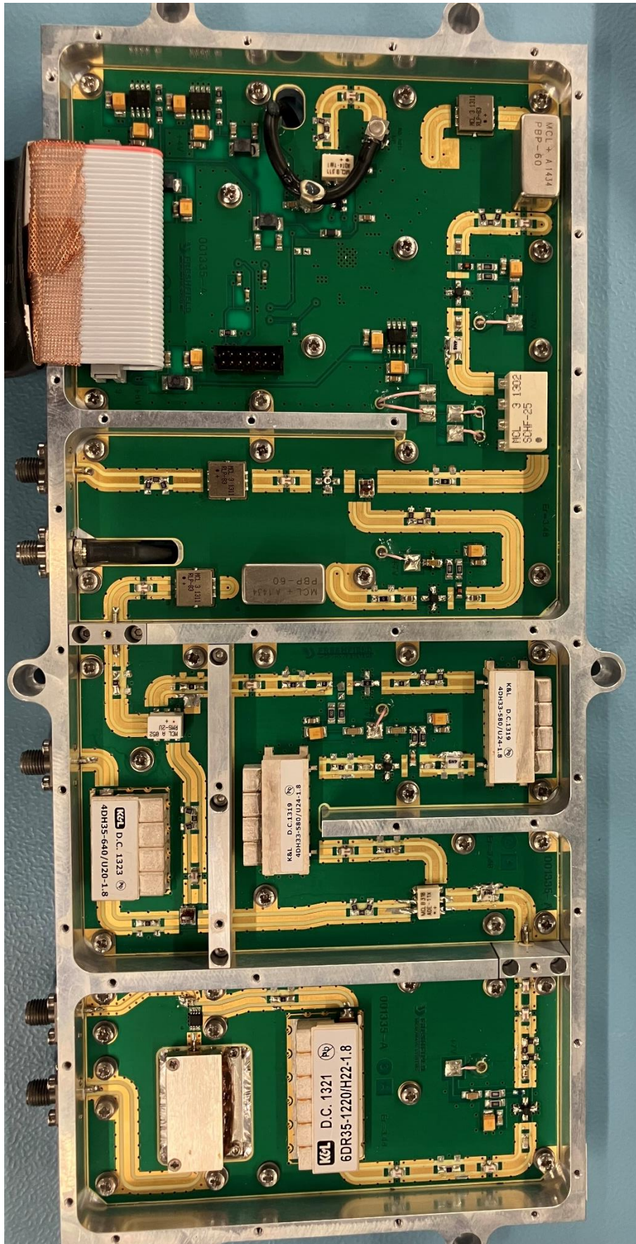
Internal – SCV A113 Downconverter (PCB 001335-1, -2, -3)
