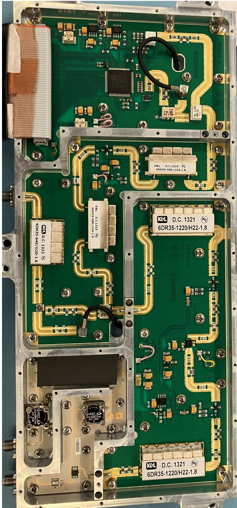
Internal – SCV Upconverter (PCB 001334-1, -2, -3, 001359-7, -9 )
