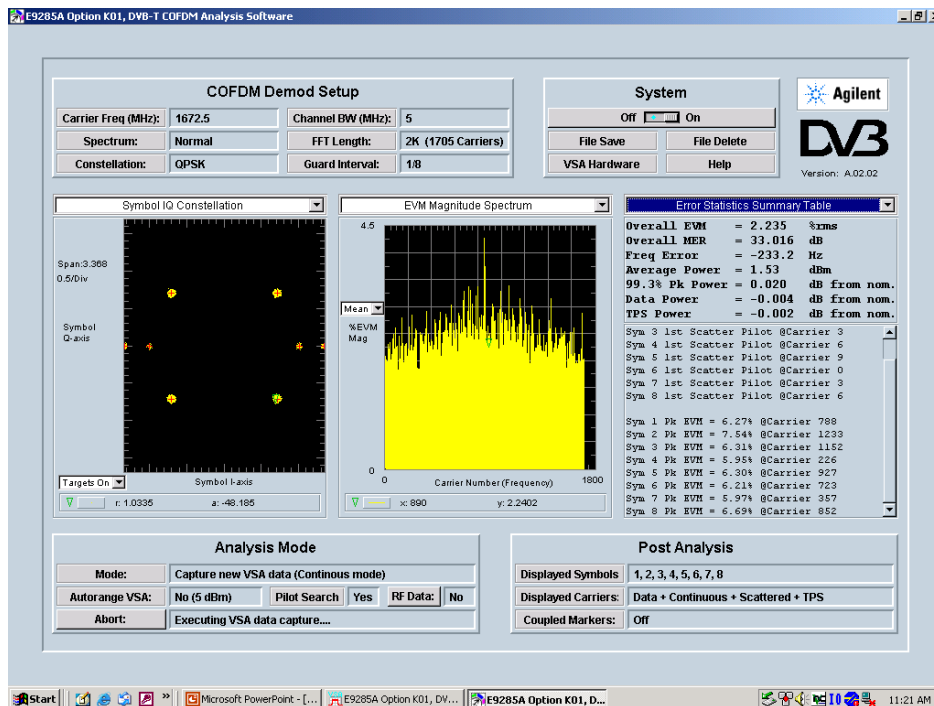
PLOT 1: Demodulation performance of the DVB-H transmitter.
