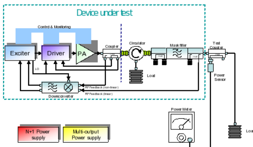
Figure 1: Test setup for RF power output measurement.
