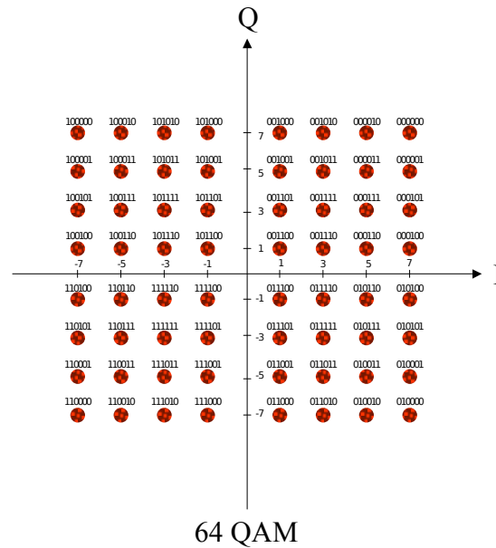
Figure 4: 64-QAM Constellation Diagram ( \alpha = 1 ).
