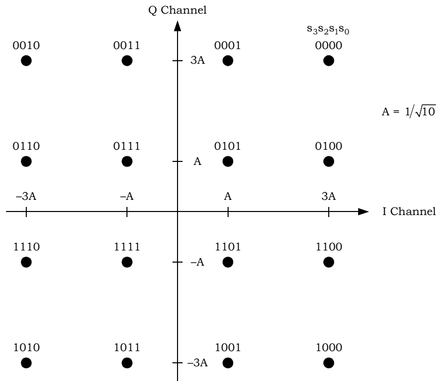
Figure 2: 16-QAM Constellation.
