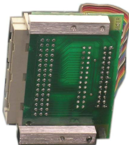
Figure 10 47266149 PCB Bottom Side View
