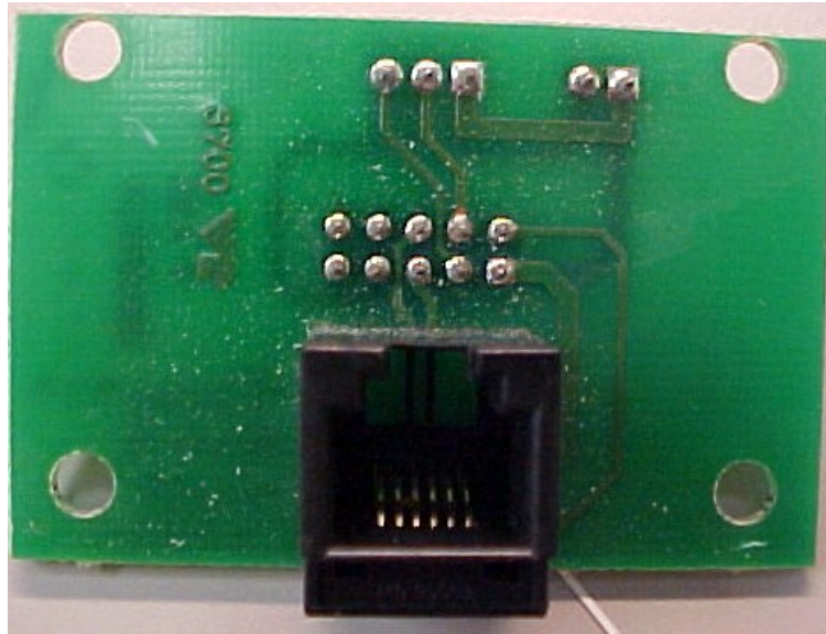
Figure 13 47266070 PCB Top Side View
