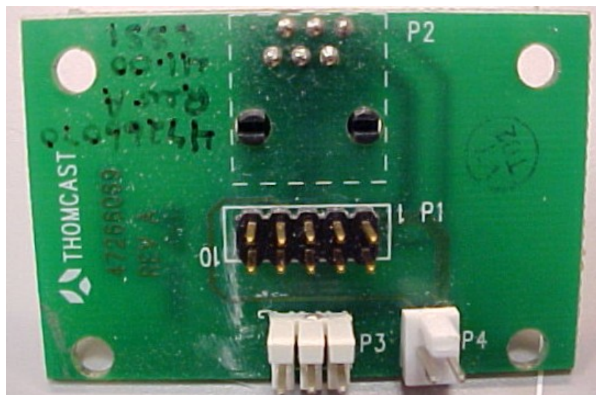
Figure 14 47266070 PCB Bottom Side View
