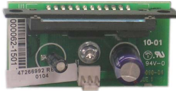
Figure 27 47266992 PCB Top Side View
