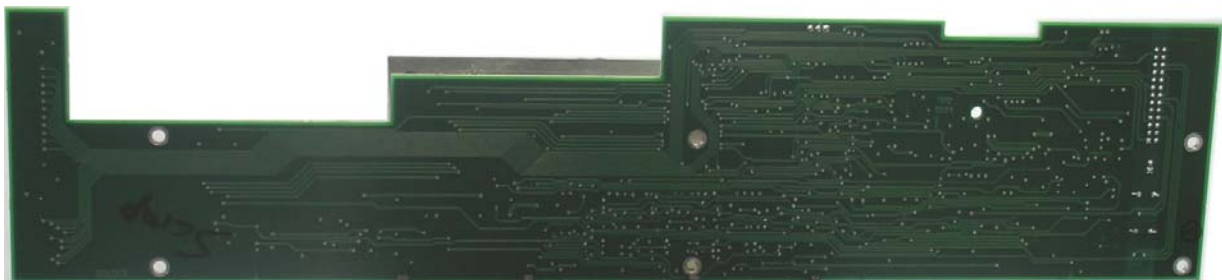
Figure 4 47267268 PCB Bottom Side View
