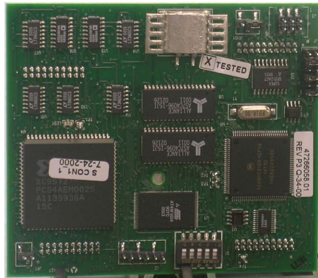
Figure 1 47266058 PCB Top Side View
