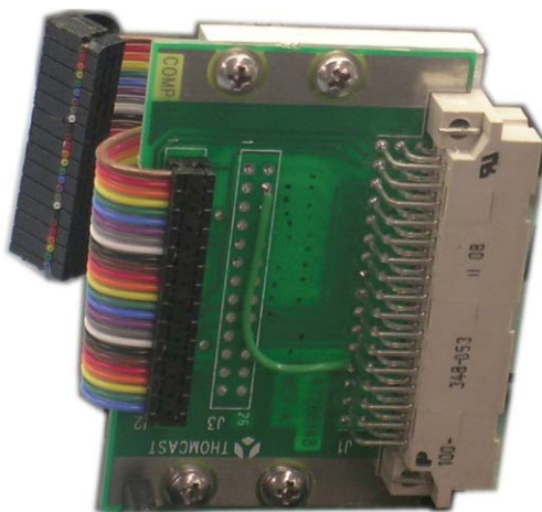
Figure 9 47266149 PCB Top Side View
