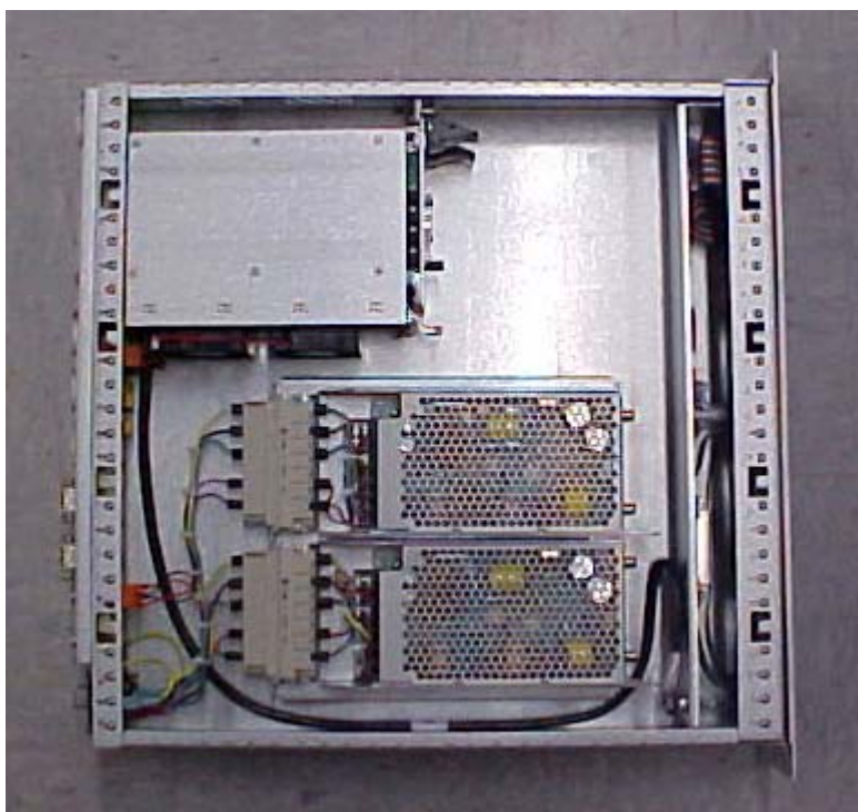
Figure 7 Dual Driver Controller (top view)
