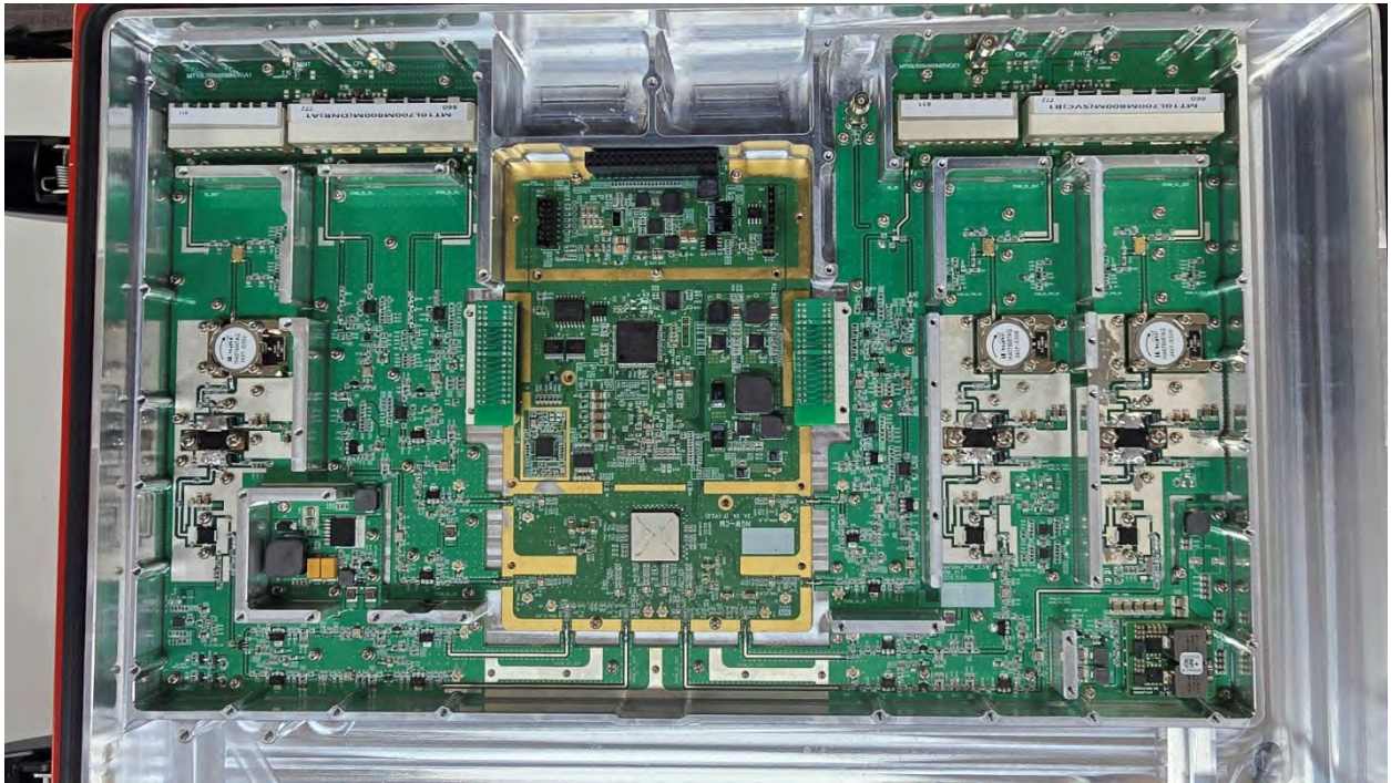
Top Shielding Covers Removed
