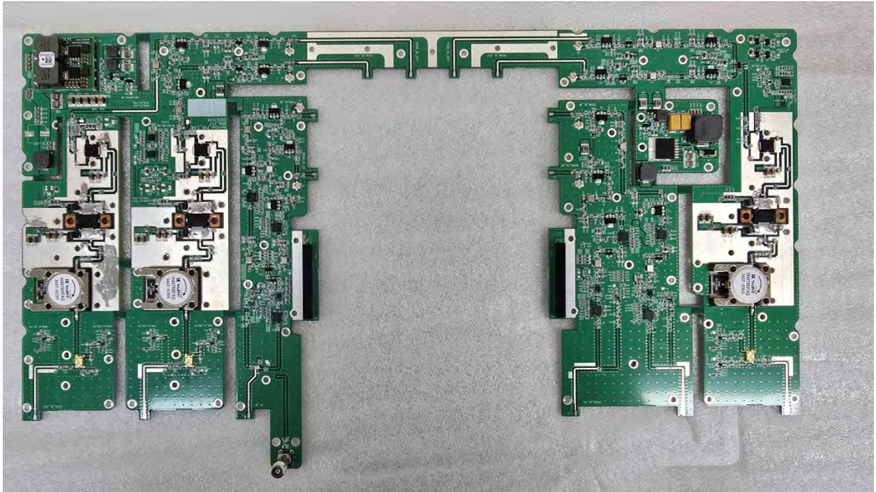
BDA PCB Bottom
