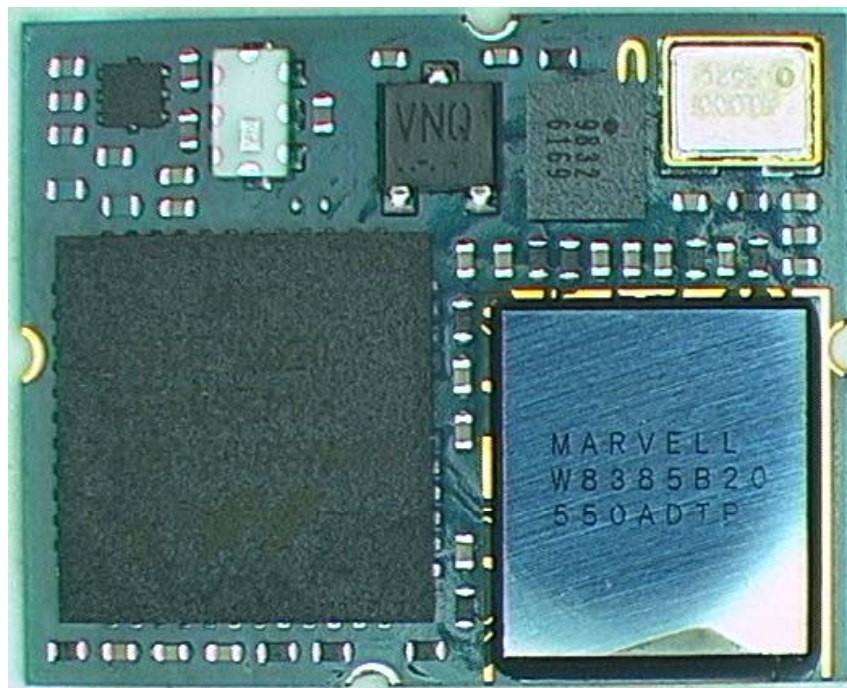
Wireless LAN Module surface (unshielded)
