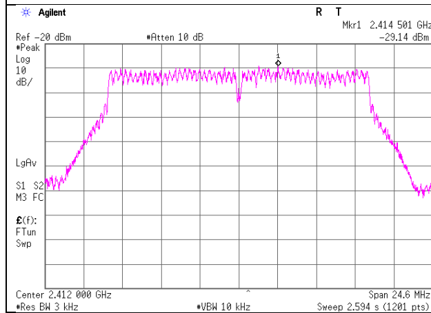
11g Antenna port 1
