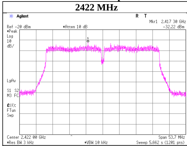
11n-40 Antenna port 1
