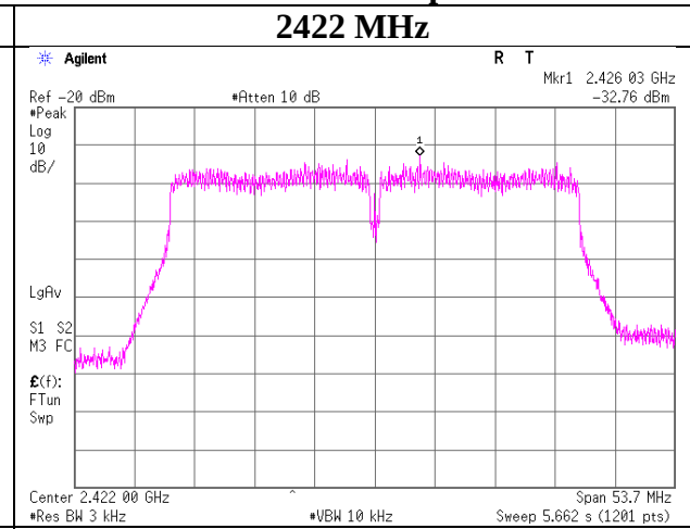
11n-40 Antenna port 2
