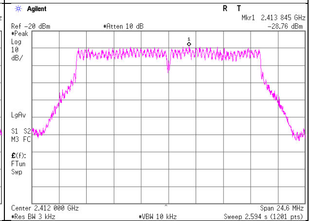
11g Antenna port 2
