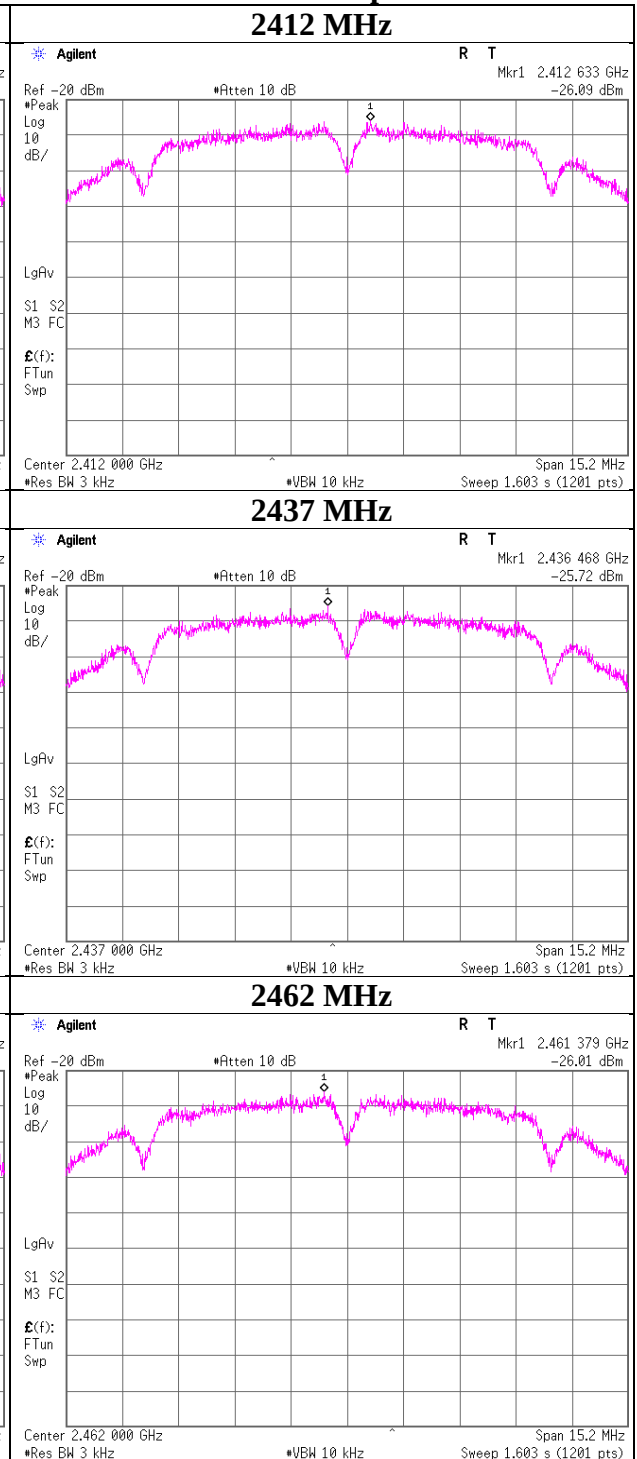
11b Antenna port 2
