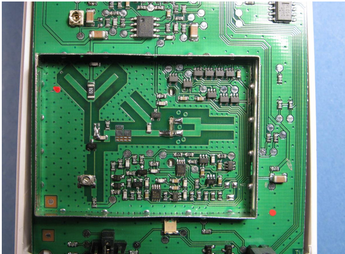
Photograph 5: - internal view of RCR-50 (in shielded enclosure)
