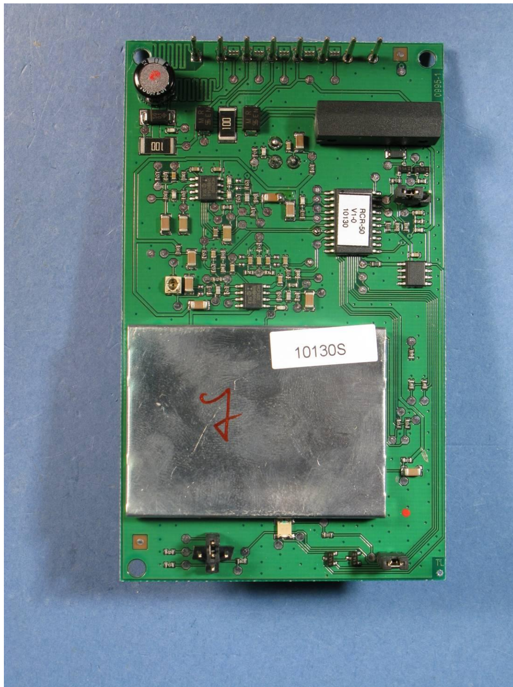
Photograph 3: - PCB view of RCR-50 (component side)
