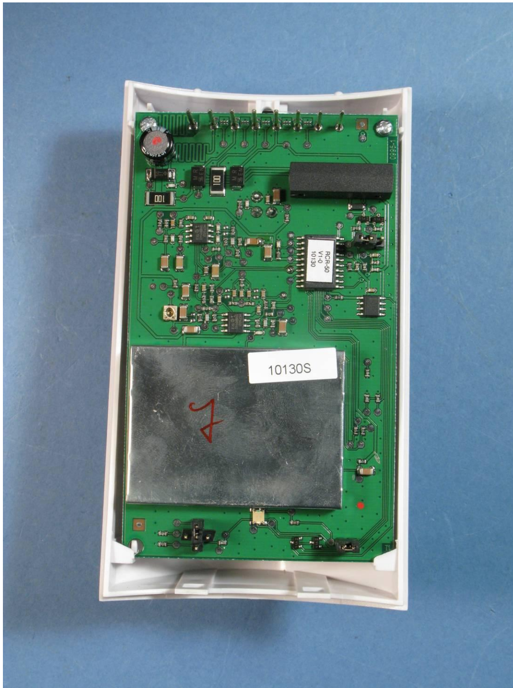
Photograph 1: - Internal view of RCR-50 (top part)
