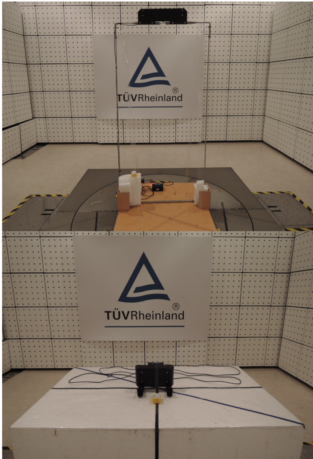
Photograph 1: Set-up for Spurious Emissions TX (Front View) Chamber
