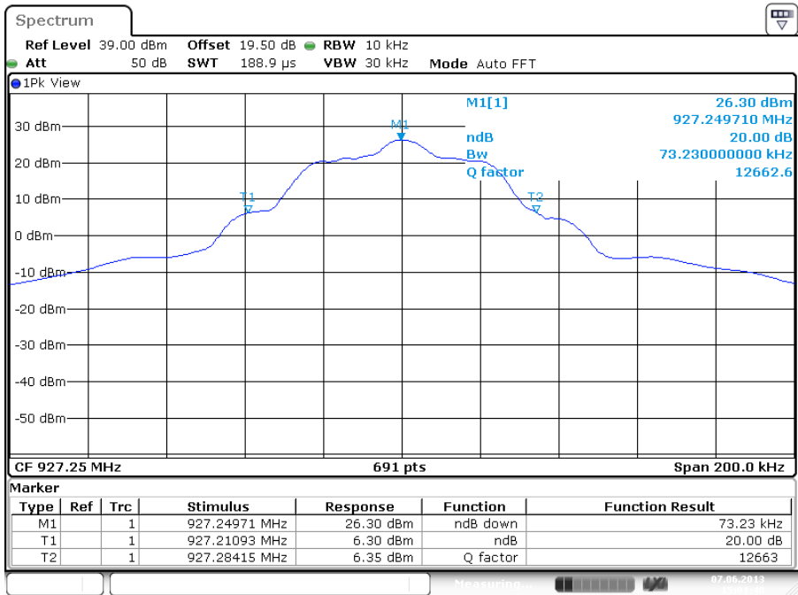
Figure 5: 20dB Bandwidth, 927.25 MHz
