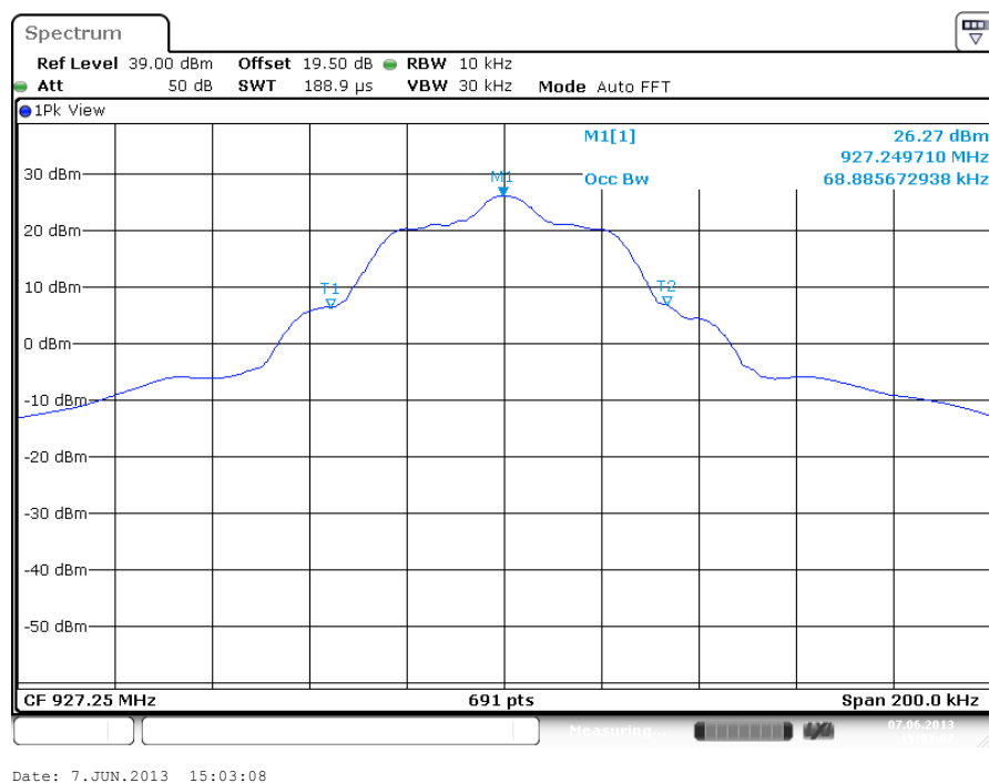
Figure 8: 99% Bandwidth, 927.25 MHz
