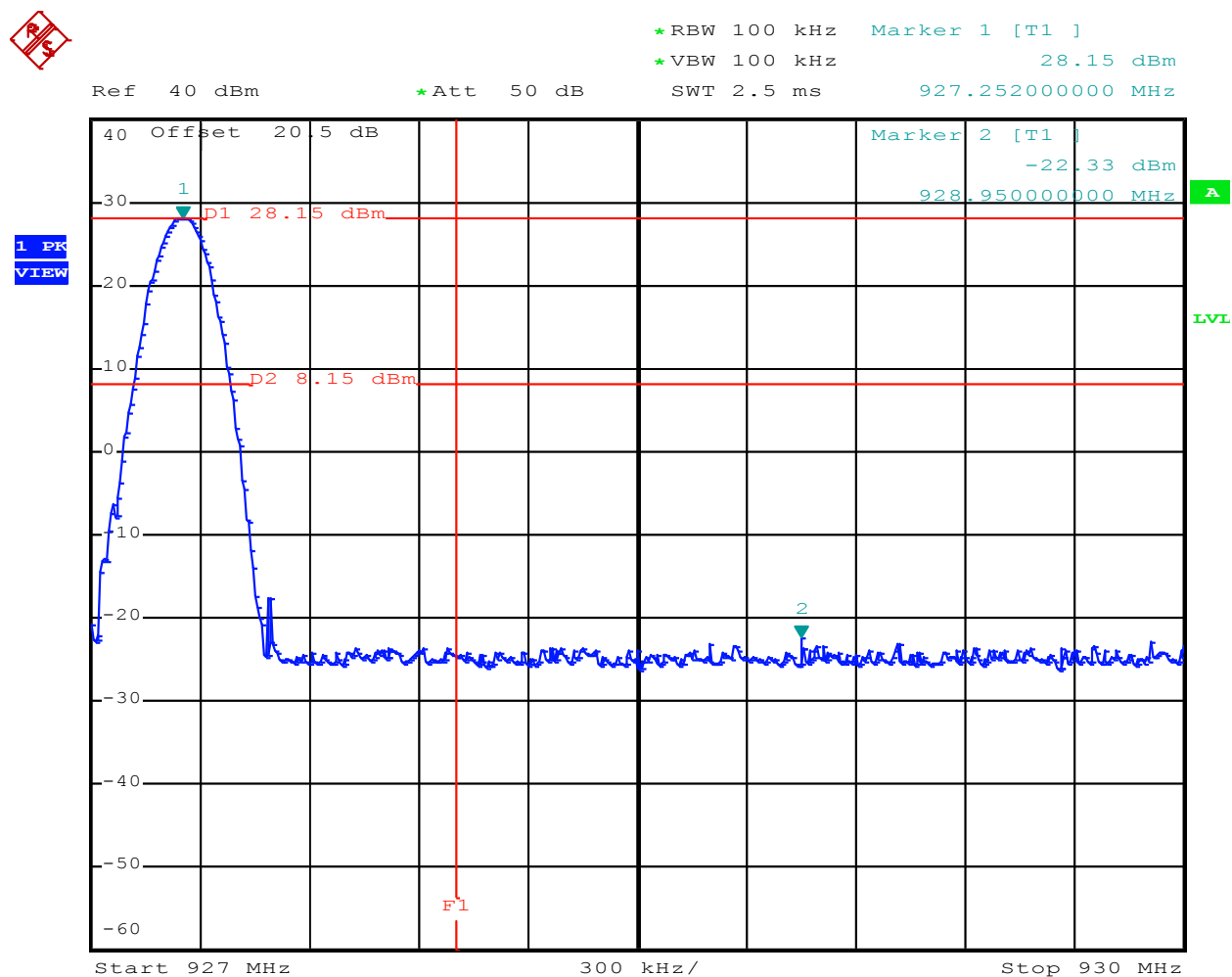
Figure 13: Band Edge Conducted Emission, Spectral Diagram, Mode: Hopping
