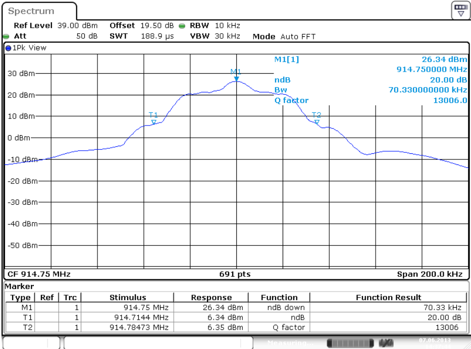
Figure 4: 20dB Bandwidth, 914.75 MHz
