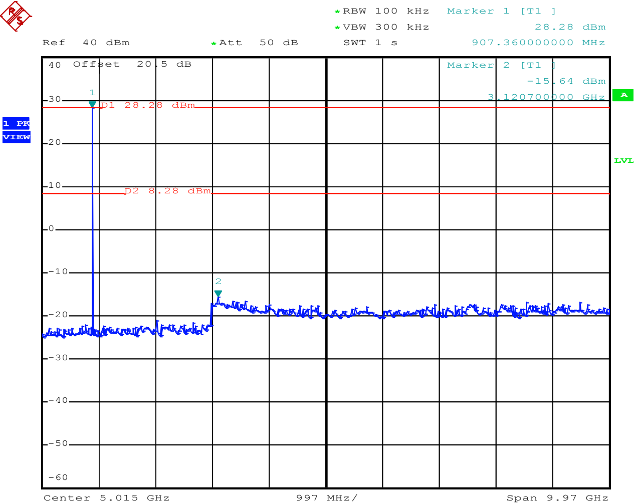
Figure 10: Conducted Spurious Emission, 30MHz - 10GHz, 914.75 MHz
