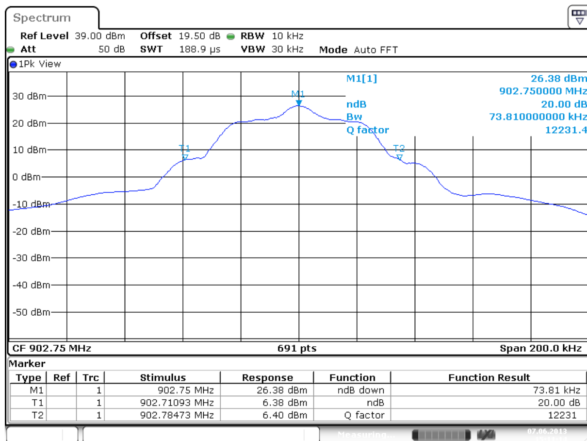
Figure 3: 20dB Bandwidth, 902.75 MHz
