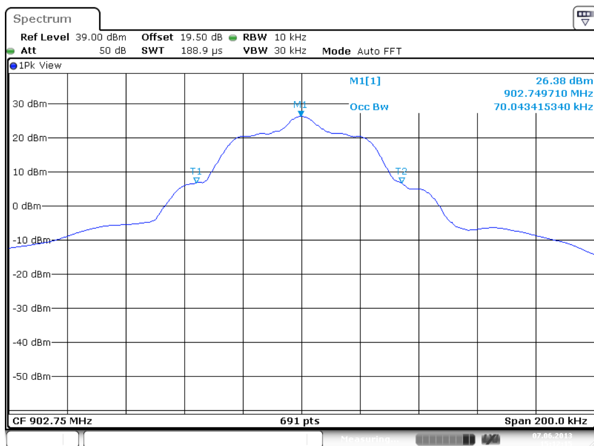
Figure 6: 99% Bandwidth, 902.75 MHz
