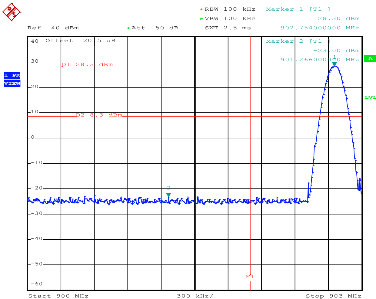
Figure 12: Band Edge Conducted Emission, Spectral Diagram, Mode: Hopping
