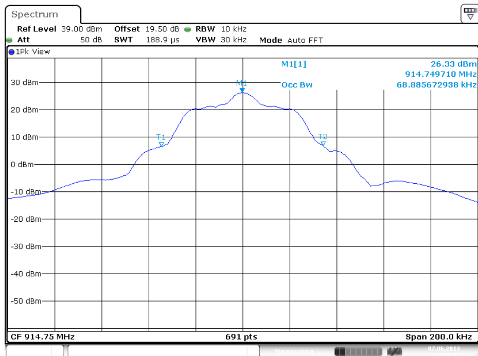
Figure 7: 99% Bandwidth, 914.75 MHz
