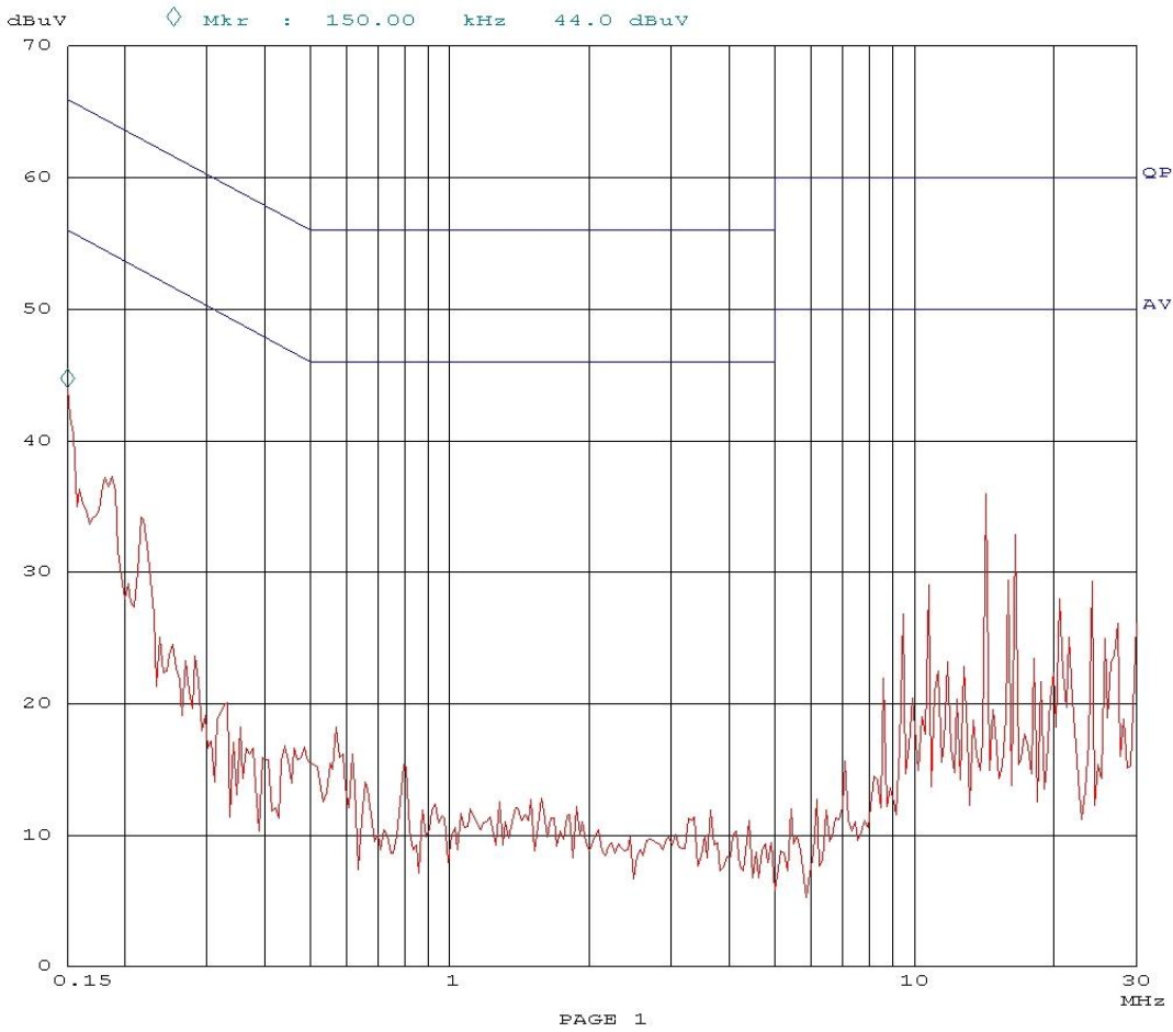
Plot 2 Conducted emissions on L2
