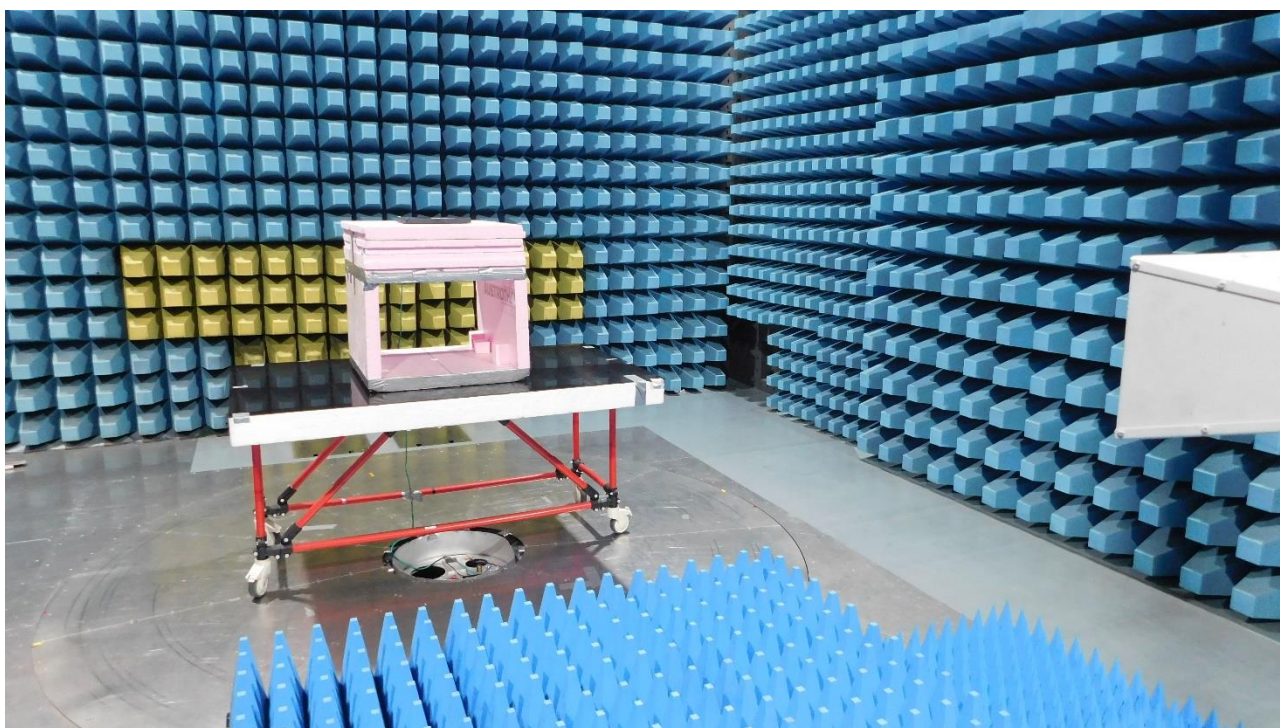
Picture 6: SAC, radiated emission test 1 GHz – 10 GHz (rear view)
