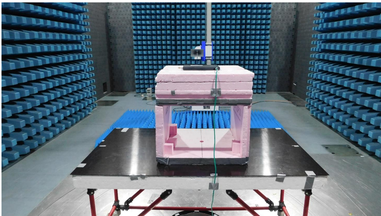
Picture 5: SAC, radiated emission test 1 GHz – 10 GHz (front view)
