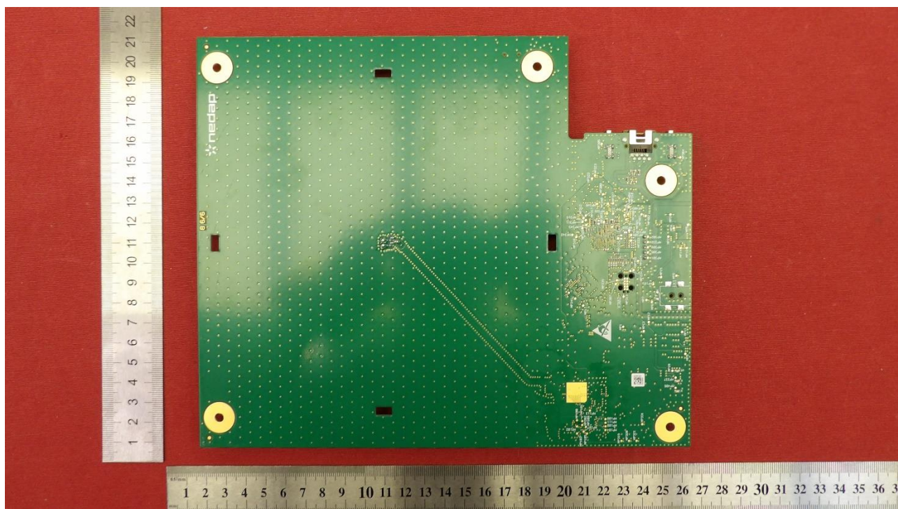
Picture 4: Main PCB of EUT – bottom side
