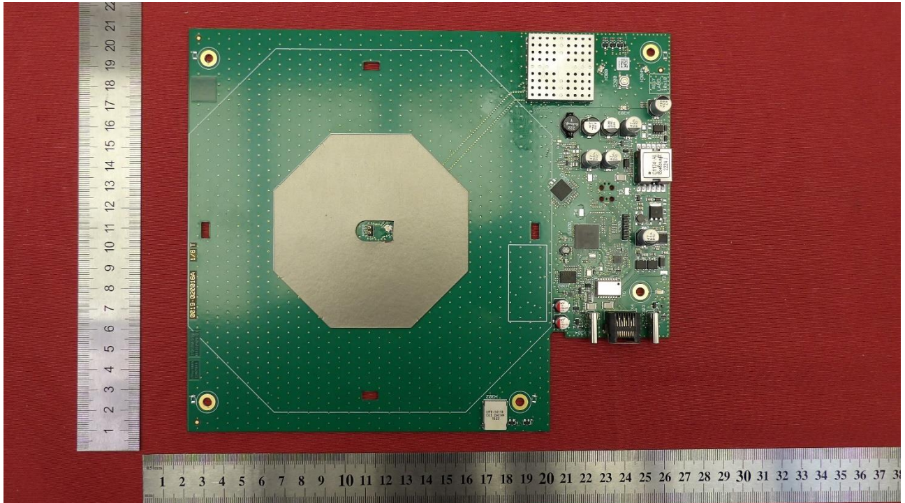
Picture 2: Main PCB of EUT - top side, with shielding
