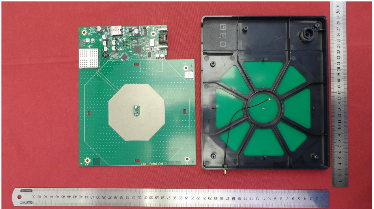
Picture 1: Main PCB of EUT with top cover
