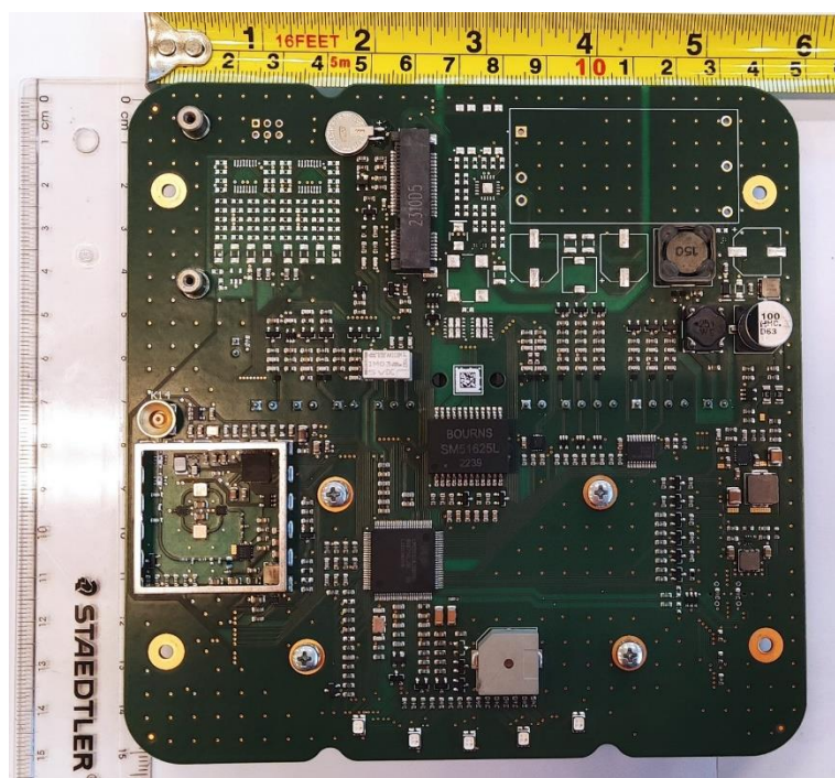
Fig.2 – Printed wiring board (main) – component side
