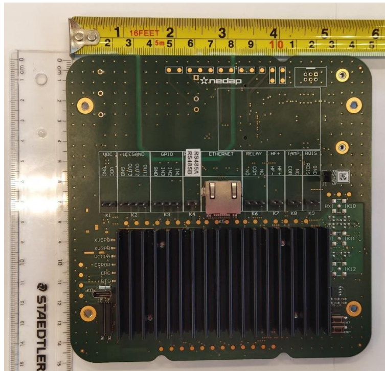
Fig.3 – Printed wiring board (main) – non-component side
