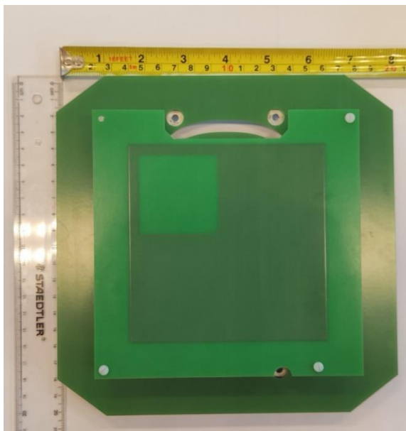
Fig.2 – PCB Primary + secondary antenna – front
