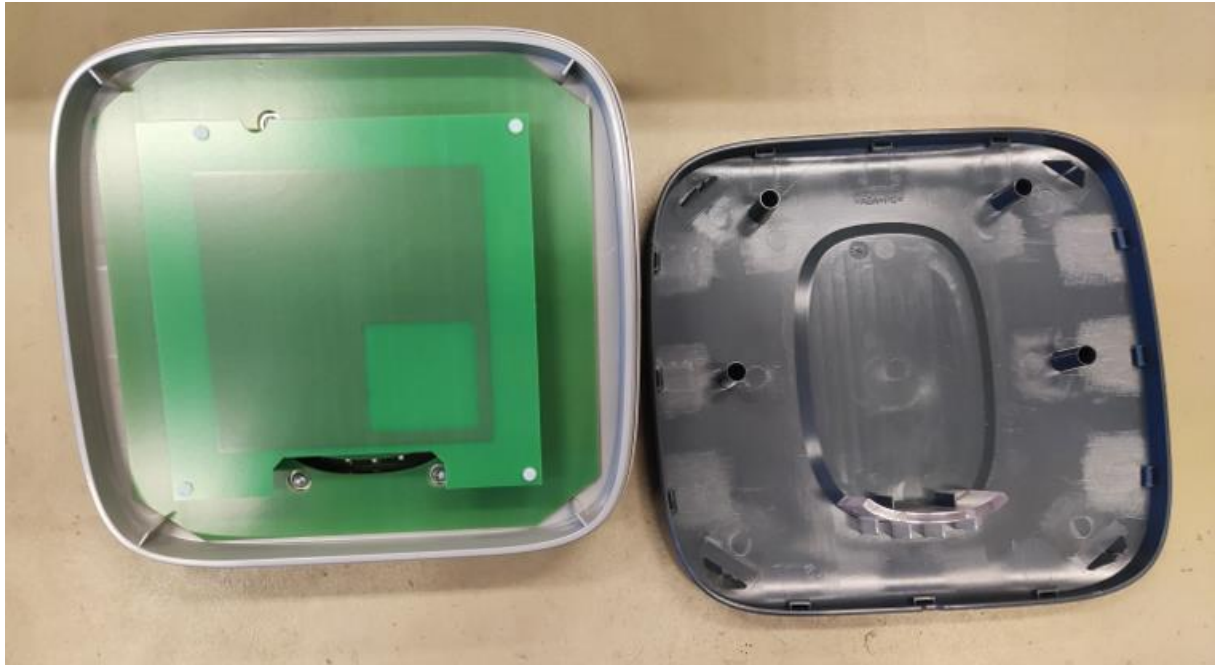
Fig.1 – Front enclosure with front cover removed (non-user accessible) and showing mounted Primary + secondary antenna PCB's
