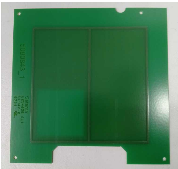
Fig.6 – PCB secondary antenna – front
