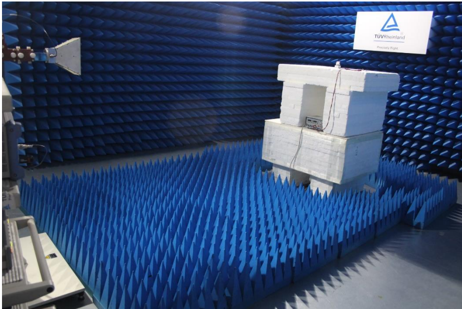
Setup 1 – 18 GHz
