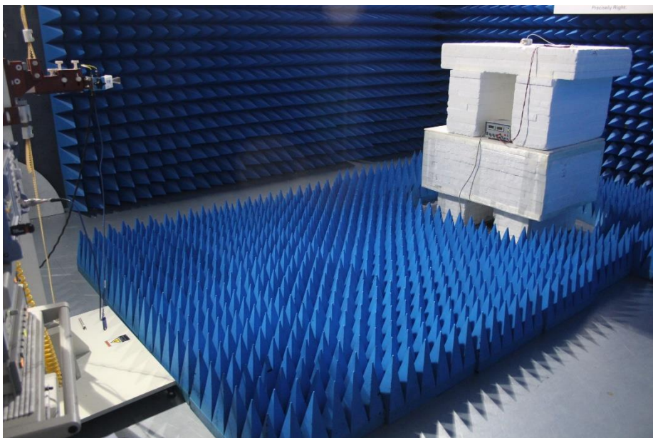
Setup 18 – 25 GHz
