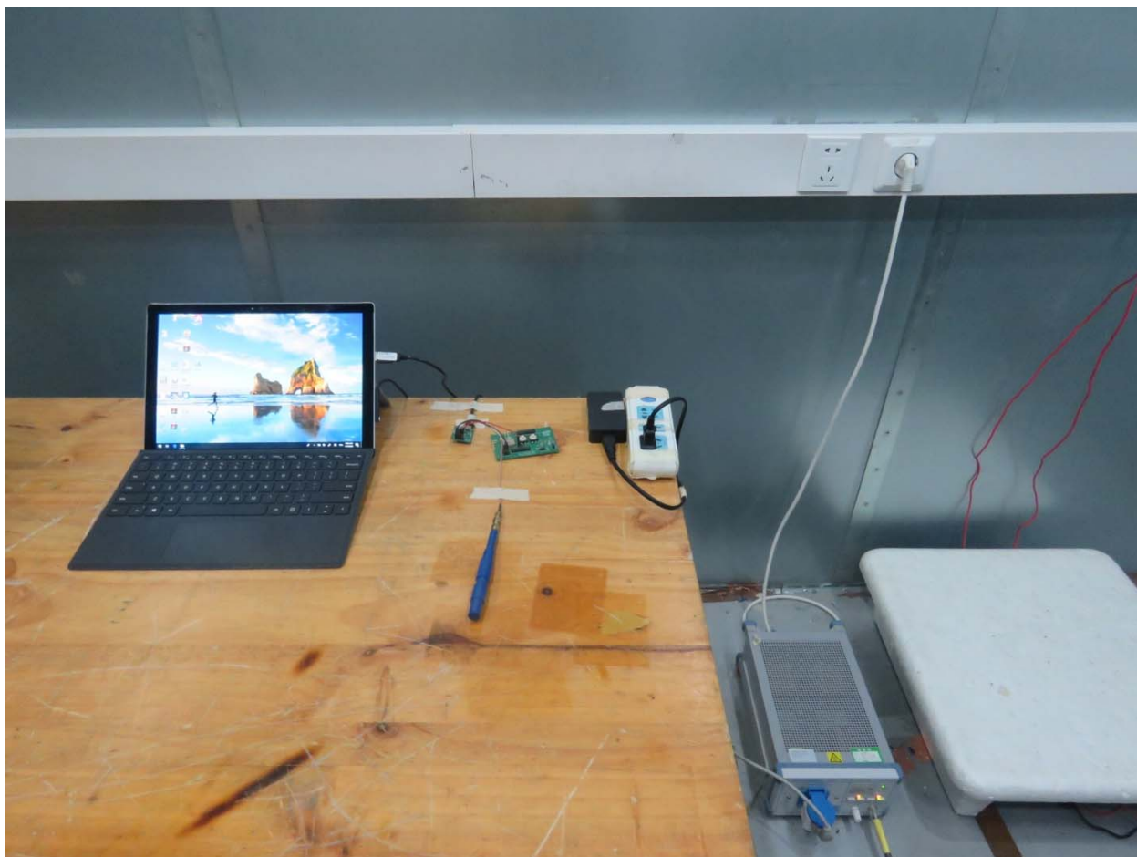
Picture 2 Conducted Emission Test Setup
