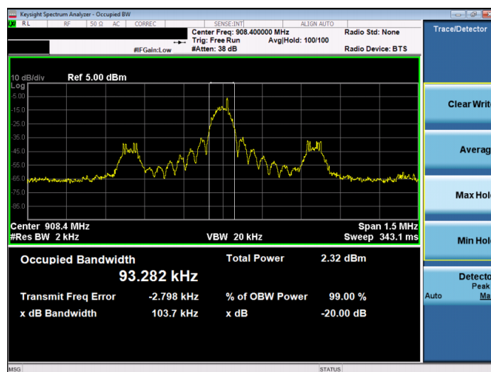
20 dB &amp; 99% Bandwidth Plot on 9.6kbps
