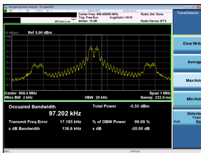
20 dB &amp; 99% Bandwidth Plot on 40kbps
