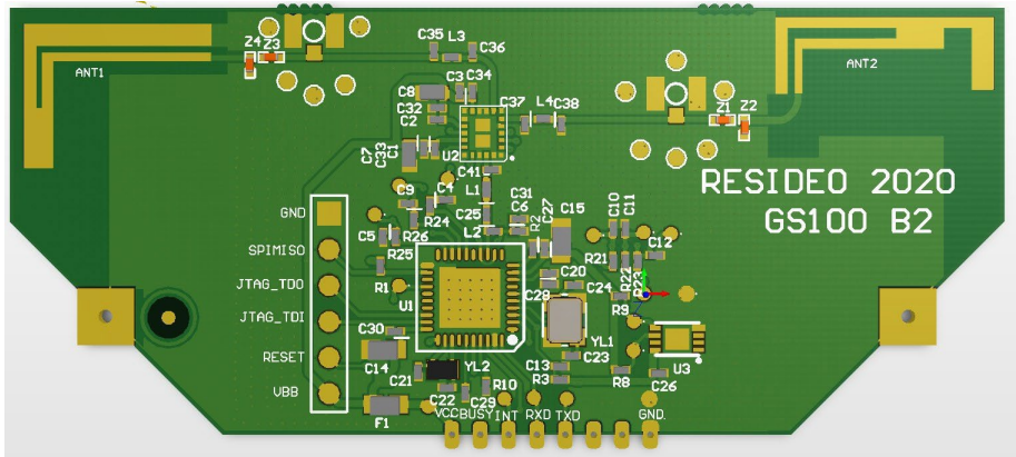
Figure 4 Daughter board with antennas
