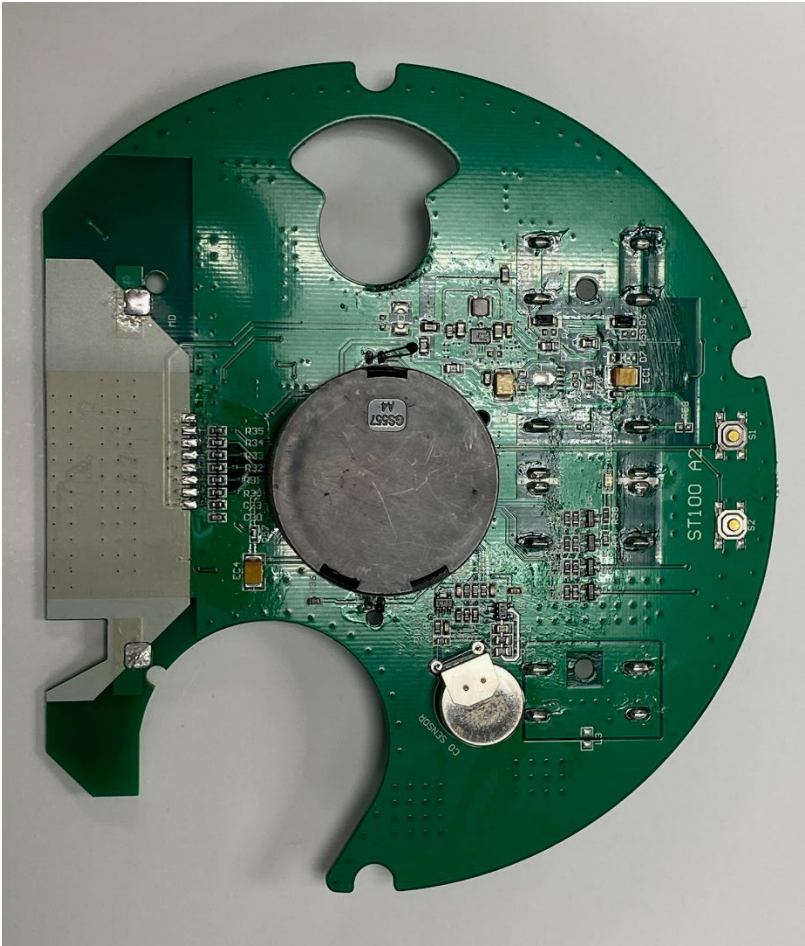
Figure 4 PCB without daughter board
