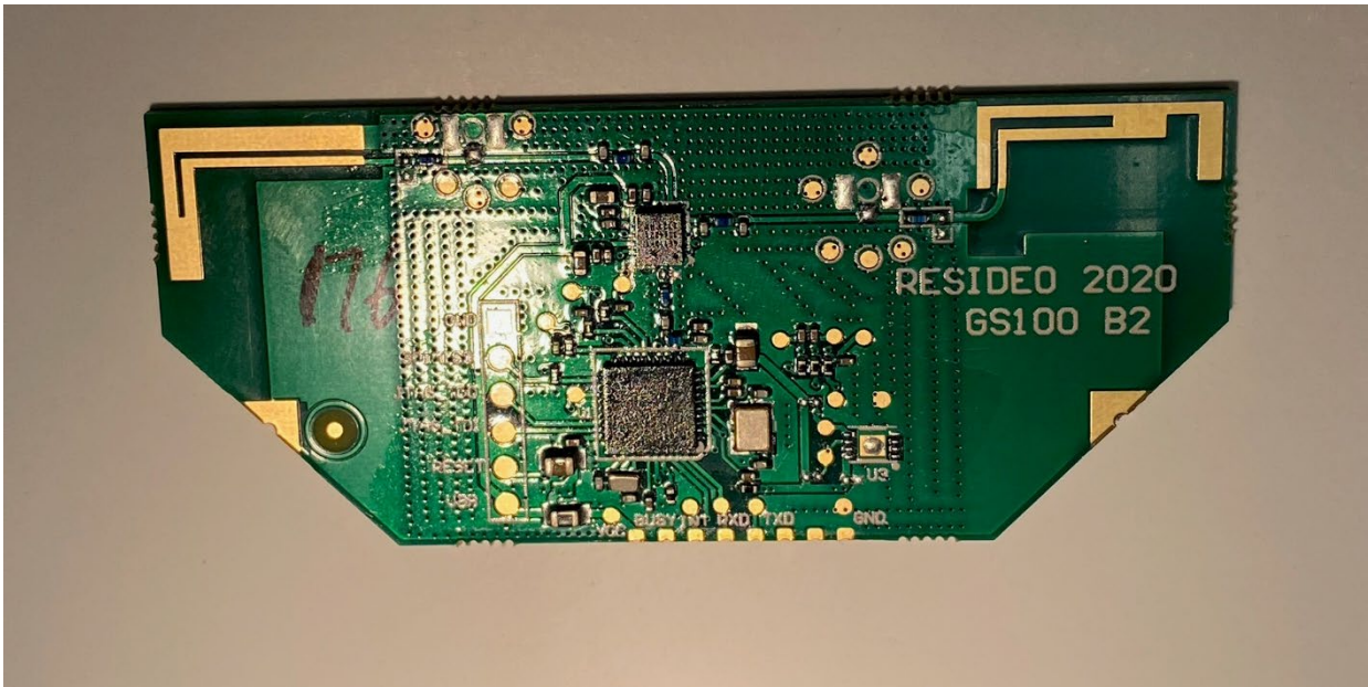
Figure 5 Daughter board top view
