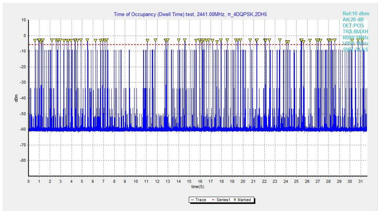
Fig. 72 Number of Transmissions ( \pi/4 DQPSK, Ch39)
