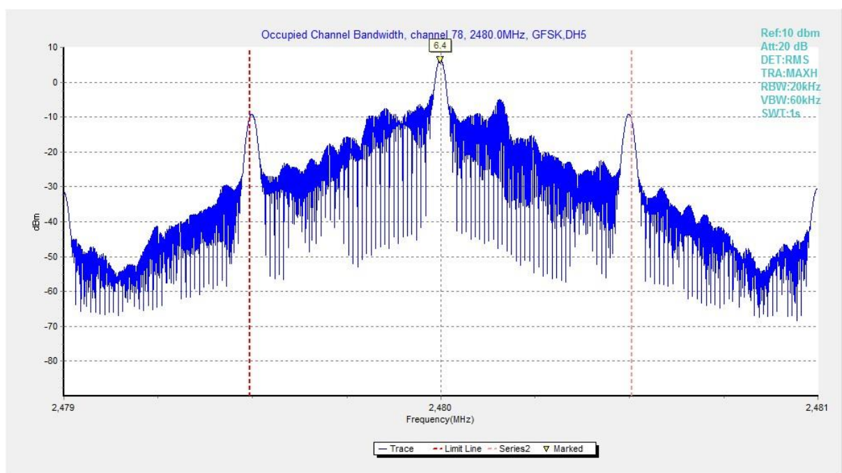
Fig. 90 Occupied Bandwidth (GFSK, Ch 78)
