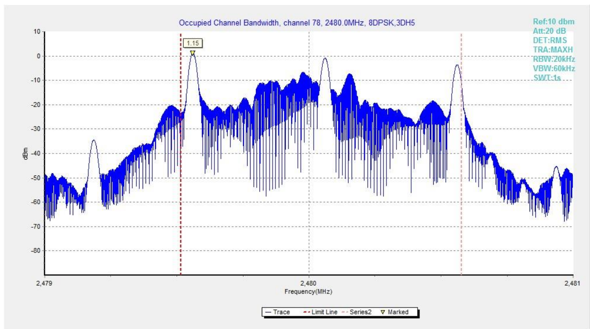
Fig. 96 Occupied Bandwidth (8DPSK, Ch 78)
