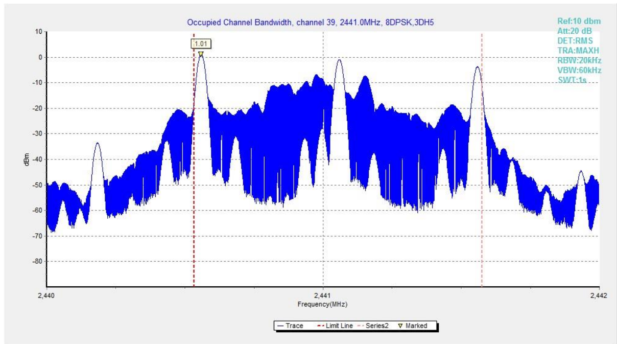
Fig. 95 Occupied Bandwidth (8DPSK, Ch 39)
