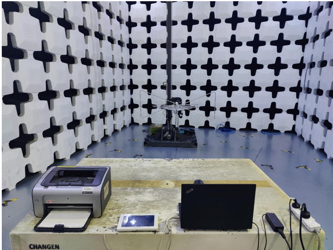
1. Radiated Emissions (Part 15B, Data Transfer, 30MHz-1GHz)
