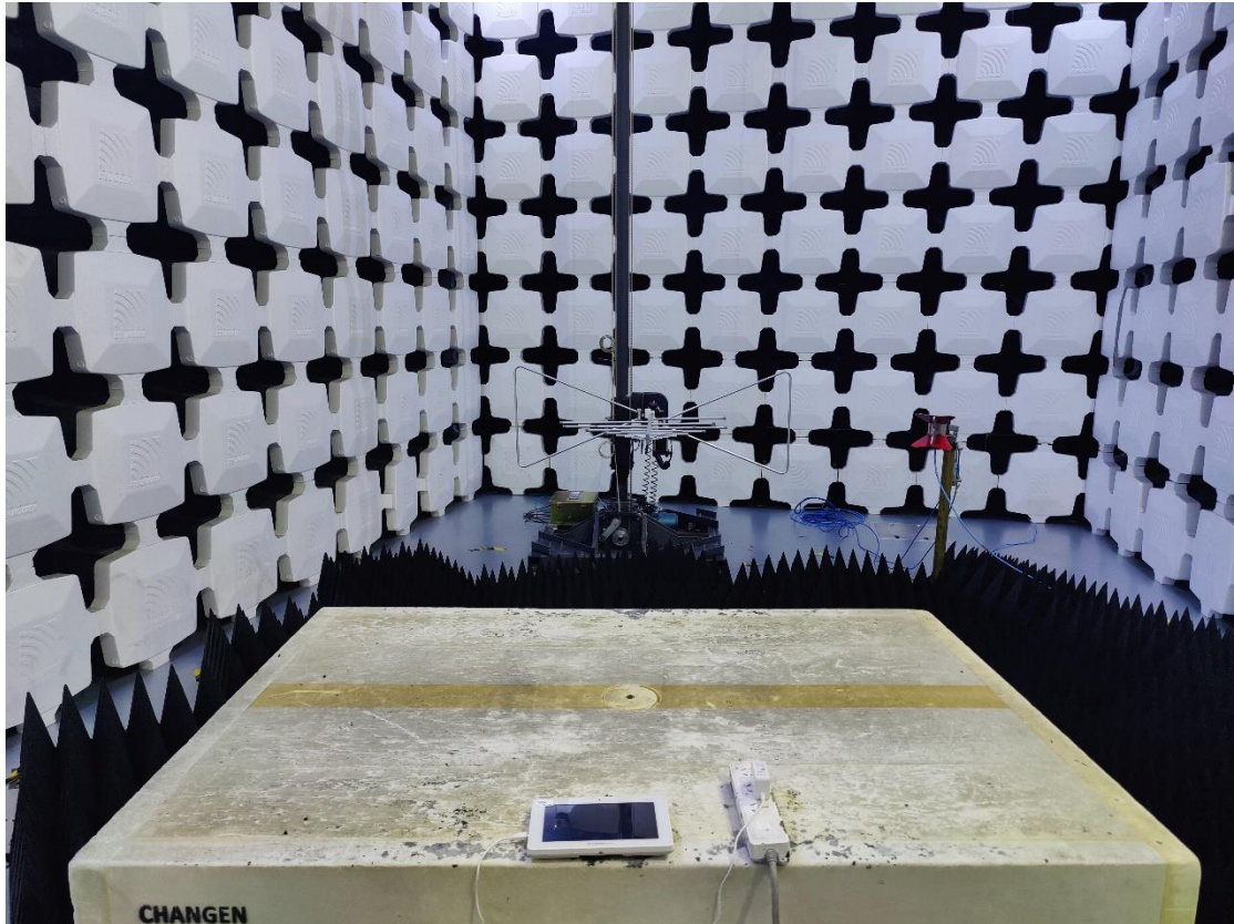
4. Radiated Emissions (Part 15B Camera, 1GHz-18GHz)
