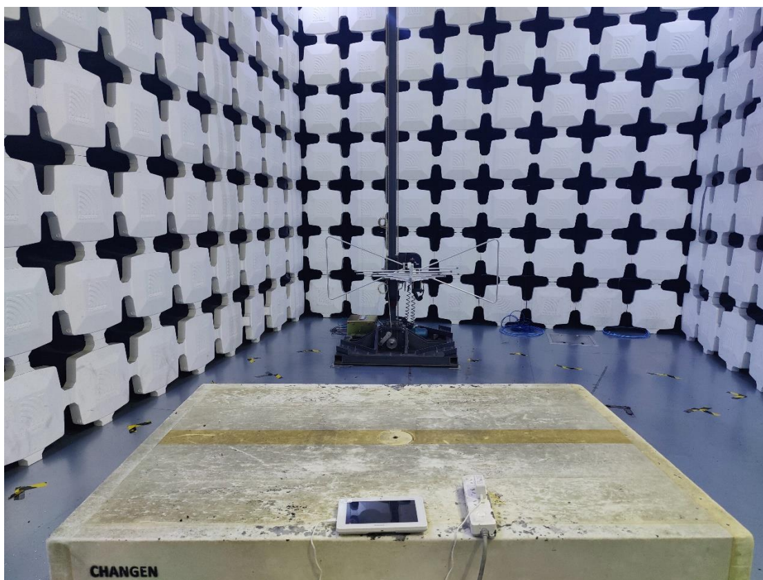
7. Radiated Emissions (Part 15C&Part 15E, 1GHz -18GHz)
