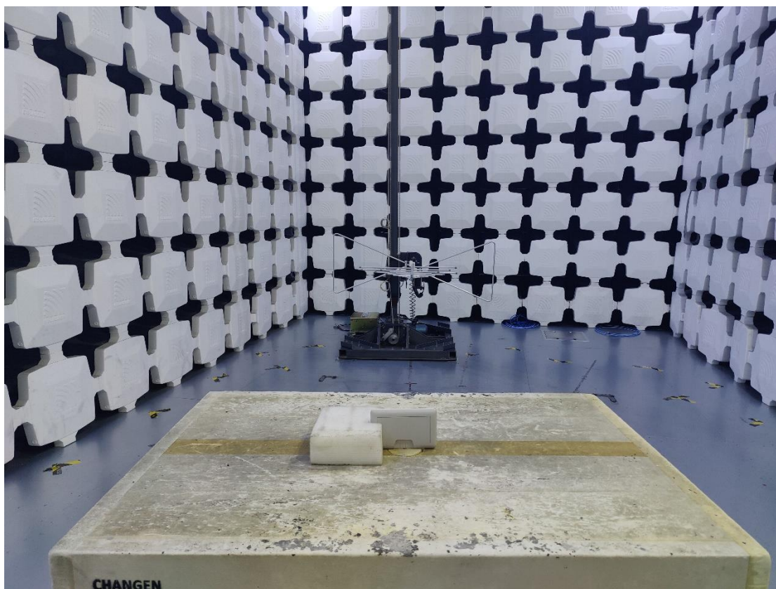
6. Radiated Emissions (Part 15C&Part 15E,30MHz-1GHz)
