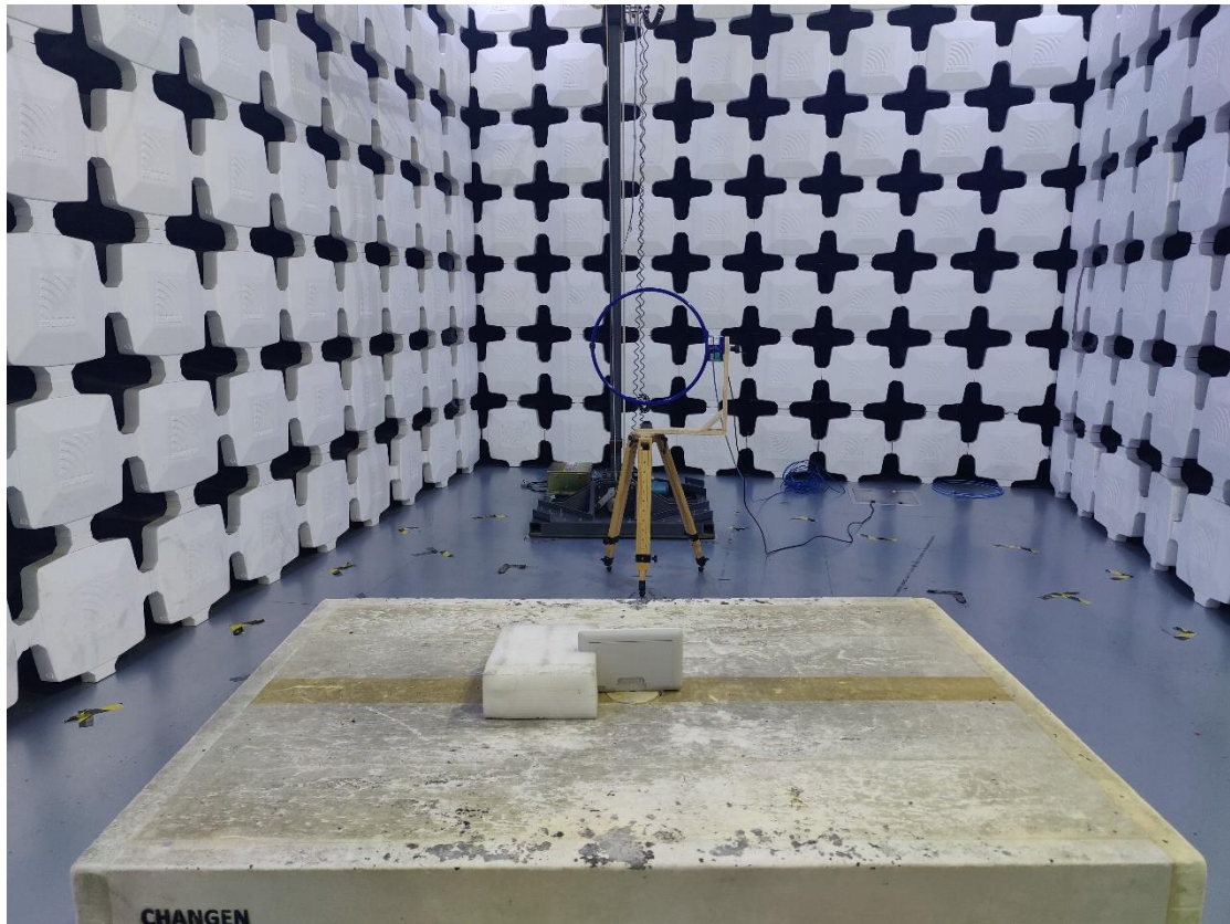
5. Radiated Emissions (Part 15C&Part 15E, 9kHz-30MHz)
