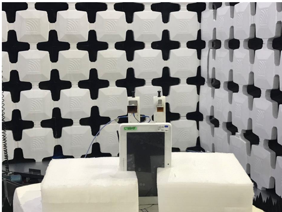
4. Radiated Emissions (Part 15C) (18-26.5GHz)
