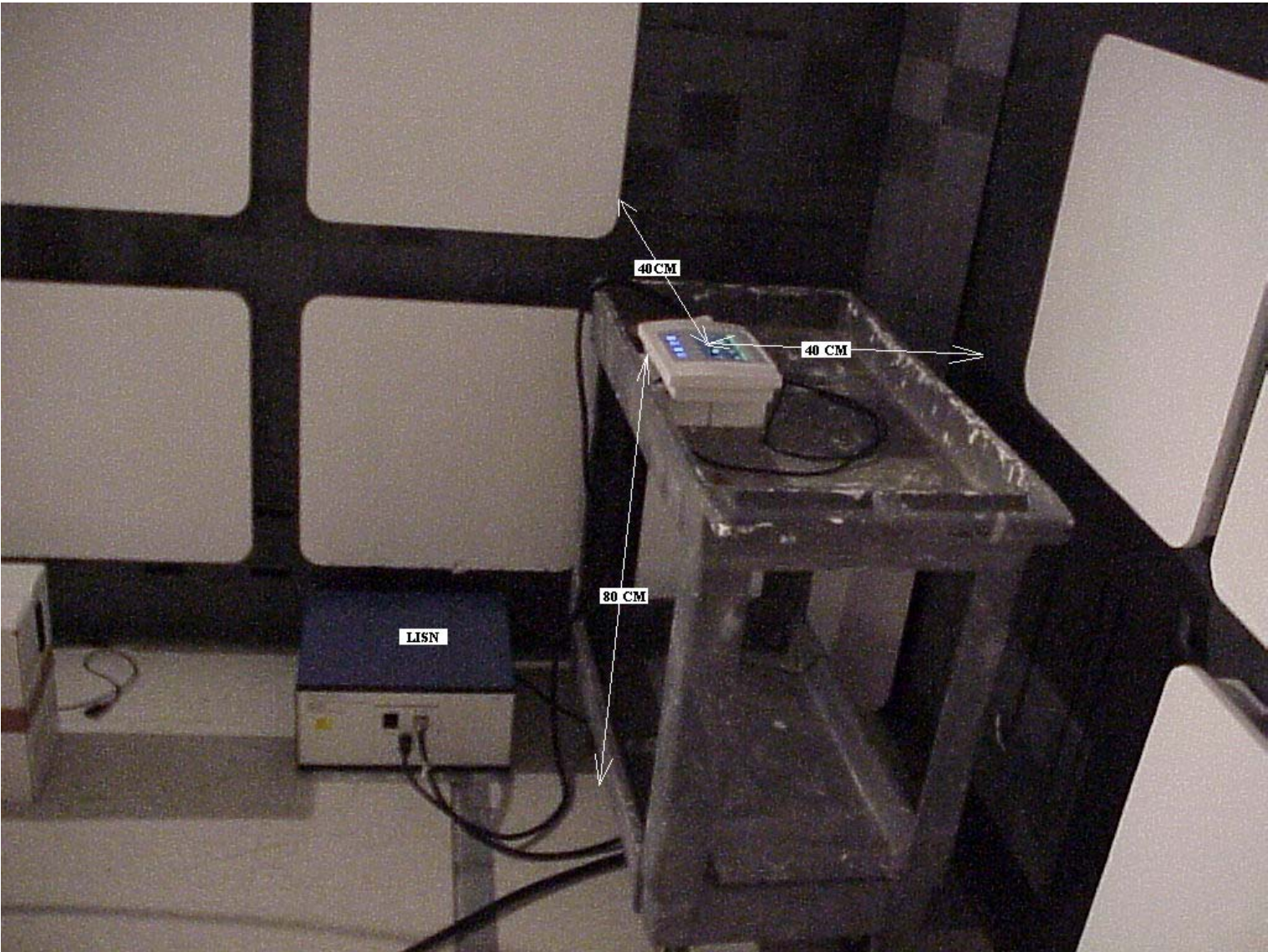
PICTURE OF LINE CONDUCTED EMISSIONS TEST
