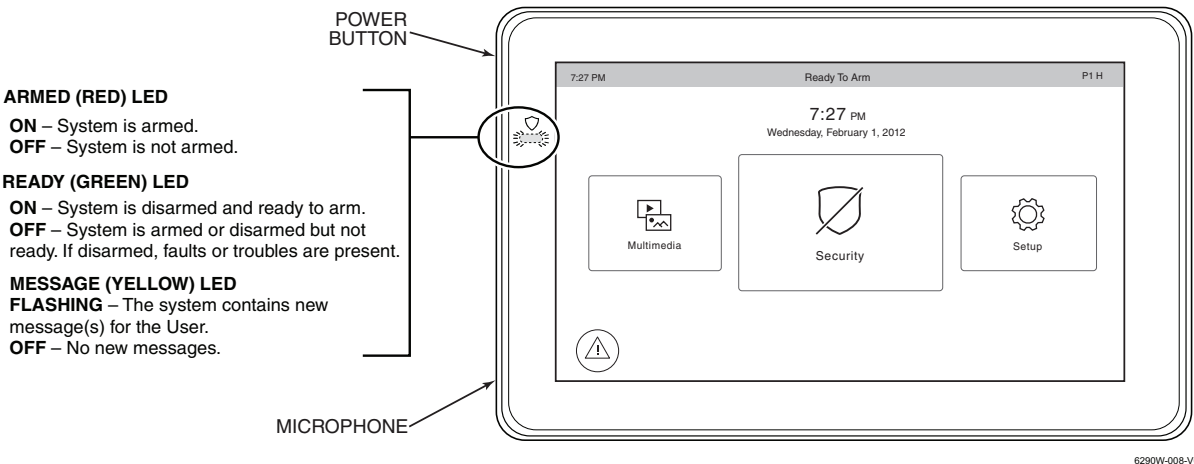
Home Screen
