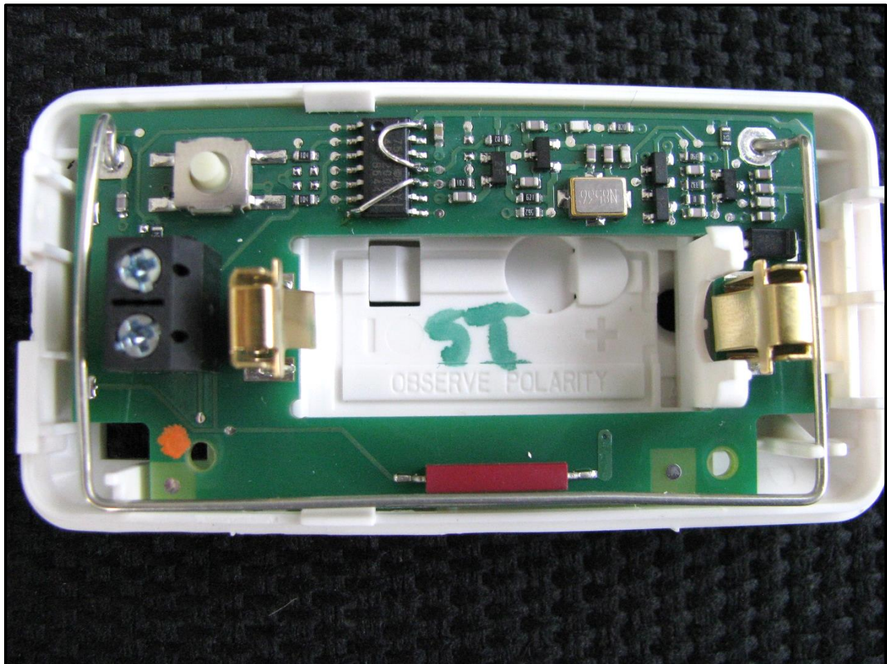
Photograph 4: EUT
