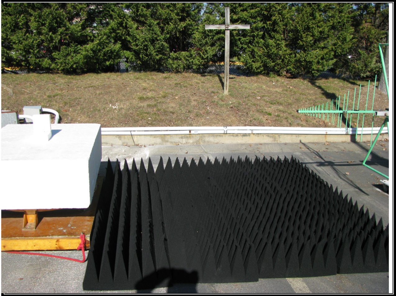
Photograph 3: Radiated Emissions
