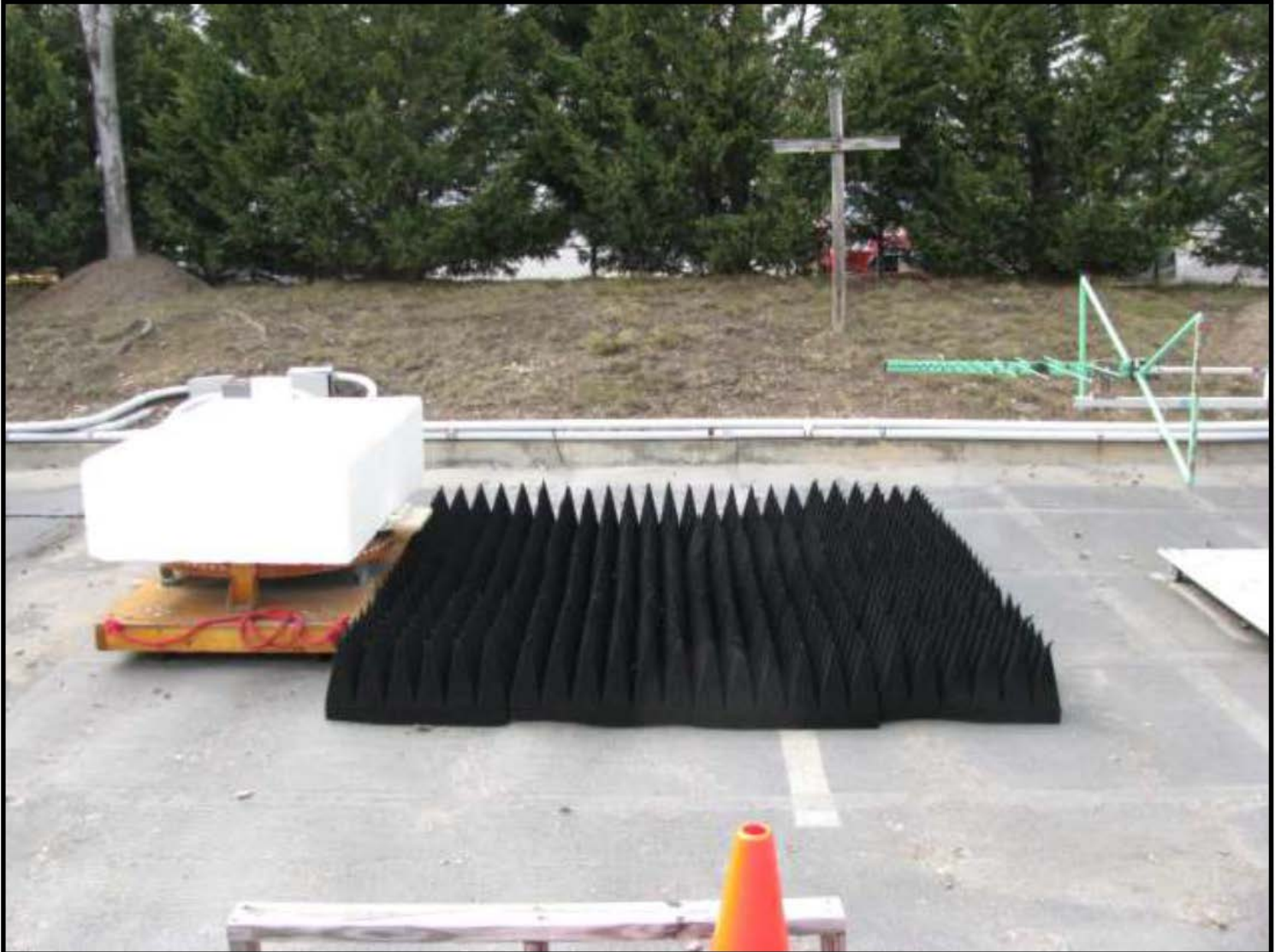
PHOTO 3: RADIATED EMISSIONS, NO TERMINATING CABLE - TEST SITE
