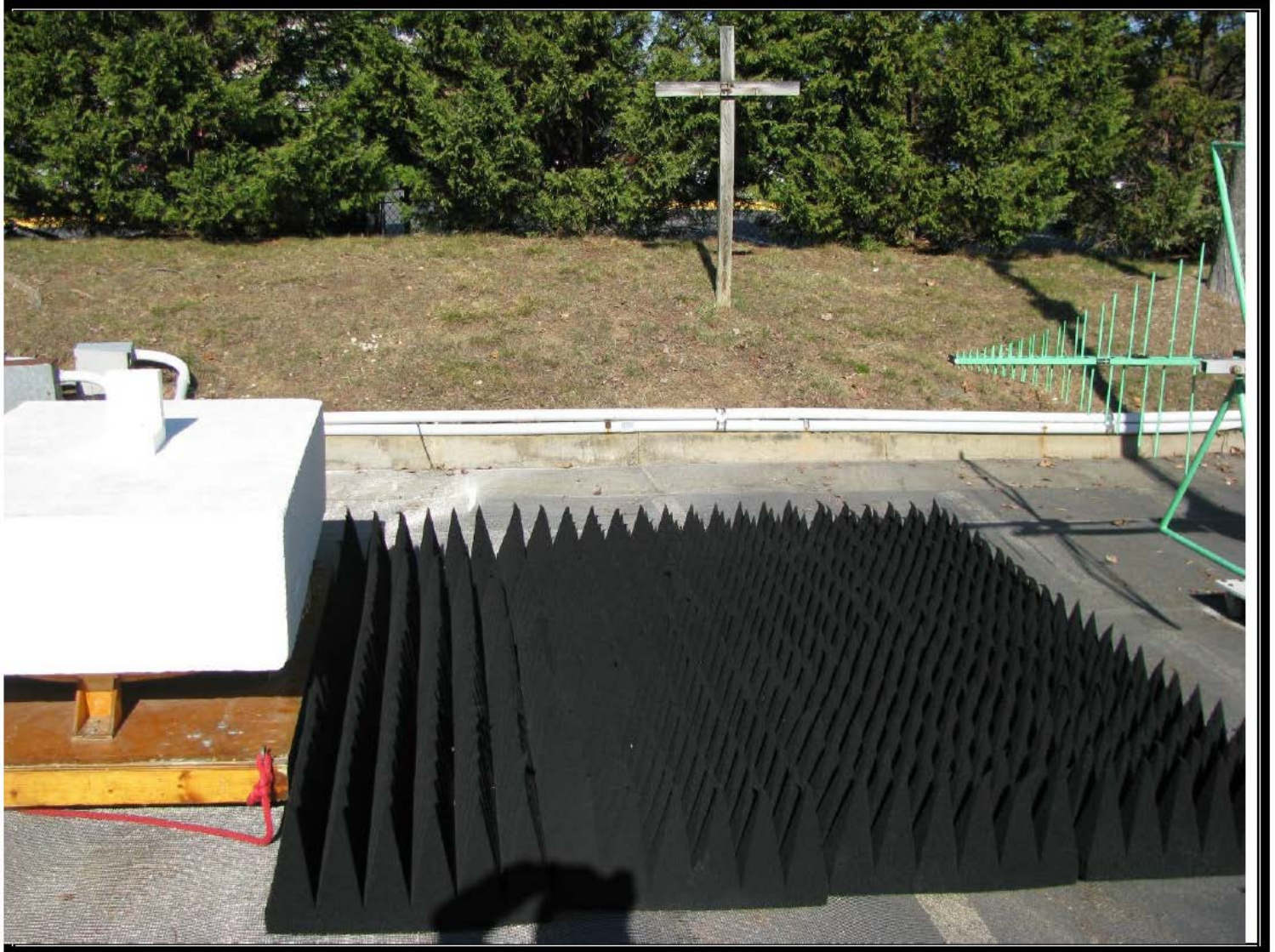
PHOTO 3: RADIATED EMISSIONS, WITH TERMINATING CABLE - TEST SITE
