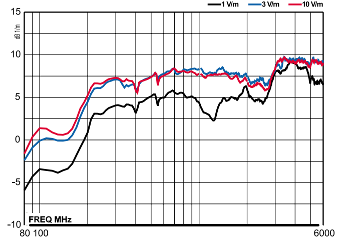
Model 3149 Gain
