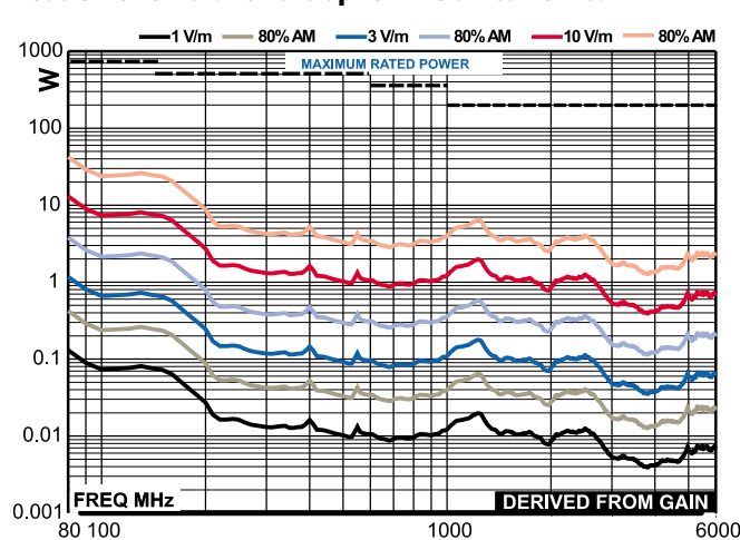
Model 3149 Forward Power Graph @ 1 m Derived from Gain
