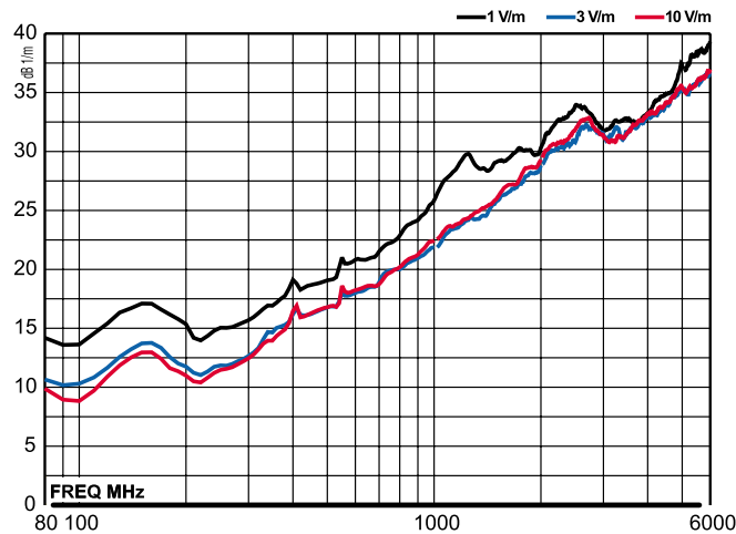
Model 3149 Antenna Factor
