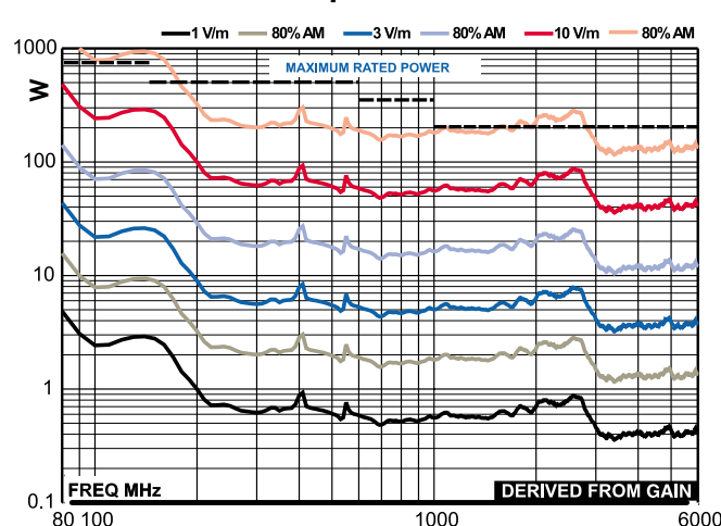
Model 3149 Forward Power Graph @ 10 m Derived from Gain
