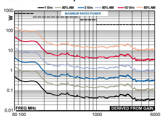
Model 3149 Forward Power Graph @ 3 m Derived from Gain
