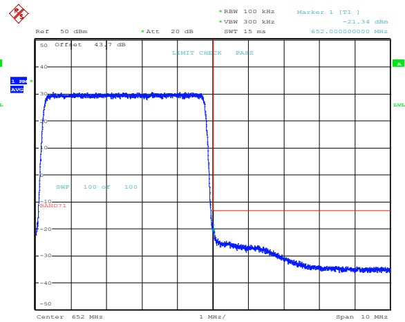
Band 71, Band Edge, 5MHz Bandwidth Setting, 256QAM
