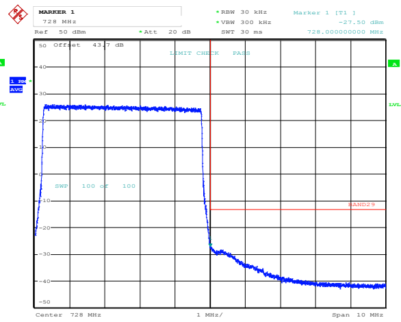
Band 29, Band Edge, 5MHz Bandwidth Setting, QPSK
