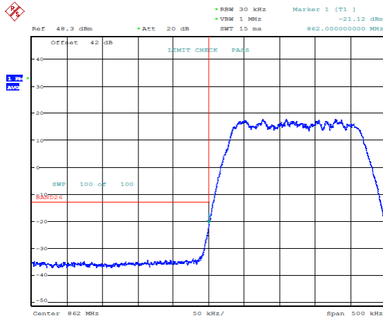
Band 26, Band Edge, NBIOT Standalone
