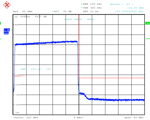
Band 71, Band Edge, 20MHz Bandwidth Setting, 64QAM
