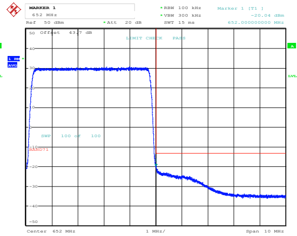
Band 71, Band Edge, 5MHz Bandwidth Setting, QPSK
