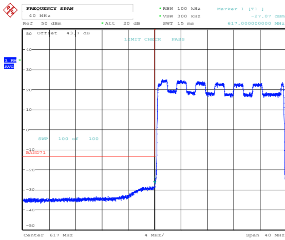
Band 71, Band Edge, 20MHz Bandwidth Setting, 16QAM
