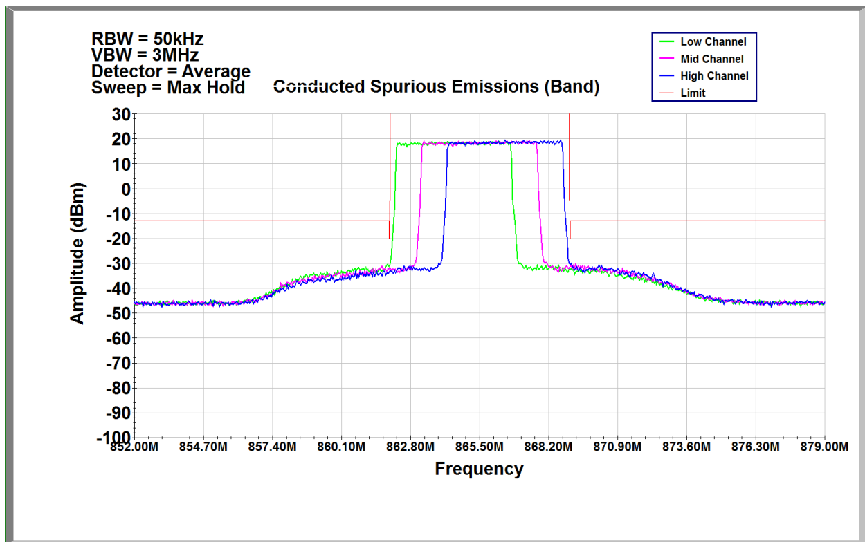
Band 26, Band Edge, 5MHz Bandwidth Setting, 64QAM (part 90.691 limit shown)
