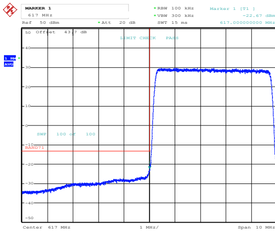
Band 71, Band Edge, 5MHz Bandwidth Setting, 256QAM
