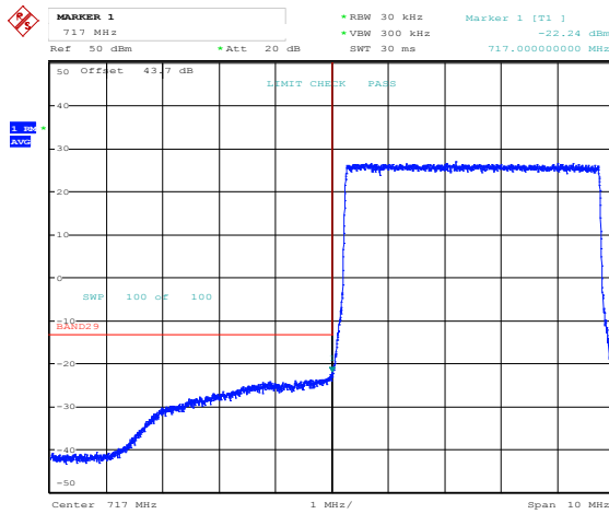
Band 29, Band Edge, 5MHz Bandwidth Setting, QPSK
