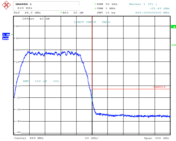
Band 26, Band Edge, NBIOT Standalone
