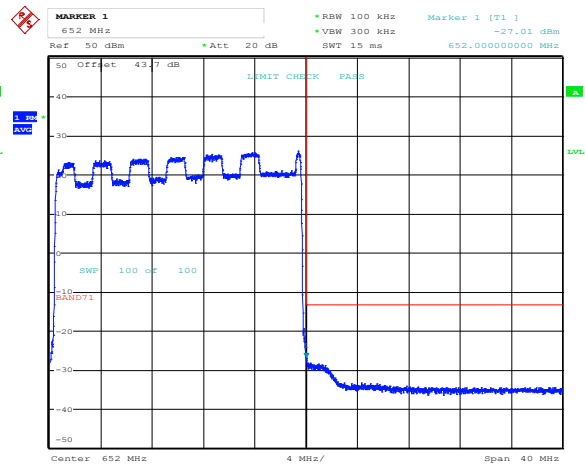
Band 71, Band Edge, 20MHz Bandwidth Setting, 16QAM
