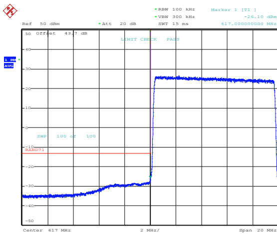
Band 71, Band Edge, 10MHz Bandwidth Setting, 64QAM
