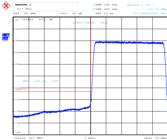
Band 71, Band Edge, 5MHz Bandwidth Setting, 64QAM
