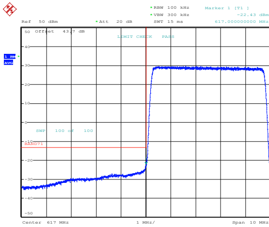
Band 71, Band Edge, 5MHz Bandwidth Setting, QPSK
