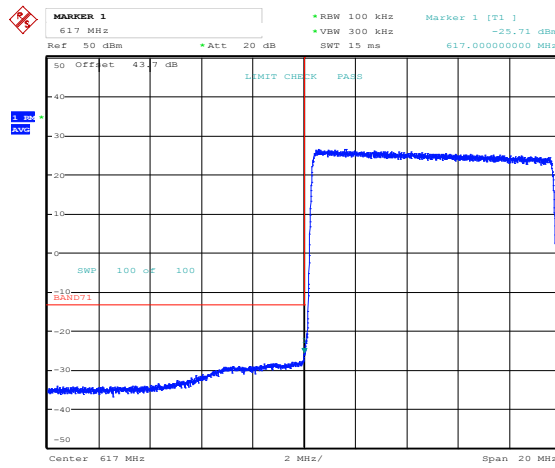
Band 71, Band Edge, 10MHz Bandwidth Setting, QPSK
