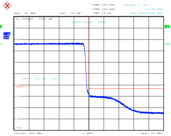
Band 71, Band Edge, 10MHz Bandwidth Setting, QPSK
