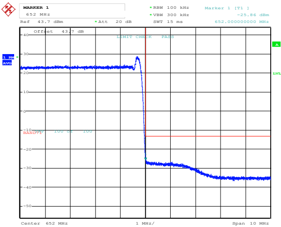
Band 71, Band Edge, NBIOT Guardband
