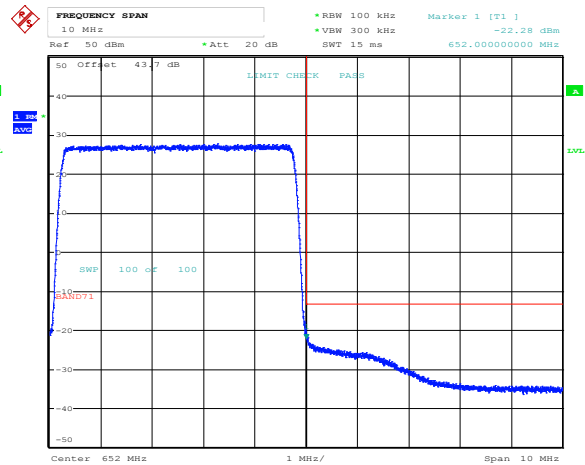
Band 71, Band Edge, 5MHz Bandwidth Setting, 64QAM
