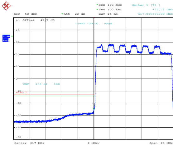
Band 71, Band Edge, 10MHz Bandwidth Setting, 16QAM
