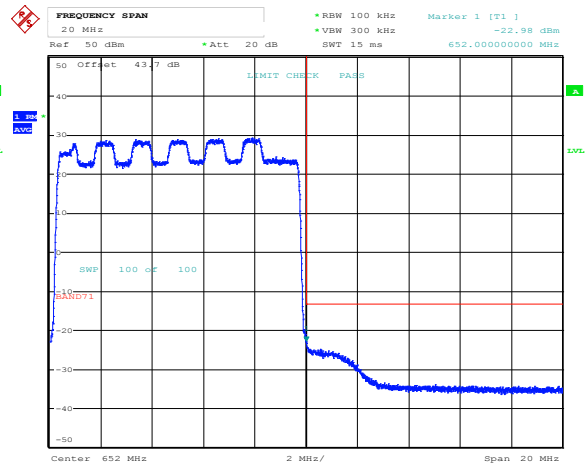
Band 71, Band Edge, 10MHz Bandwidth Setting, 16QAM
