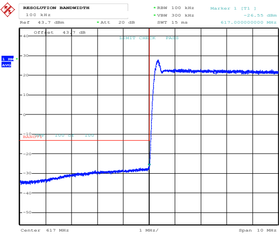
Band 71, Band Edge, NBIOT Guardband
