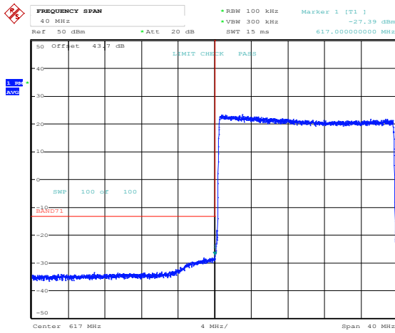
Band 71, Band Edge, 20MHz Bandwidth Setting, 64QAM
