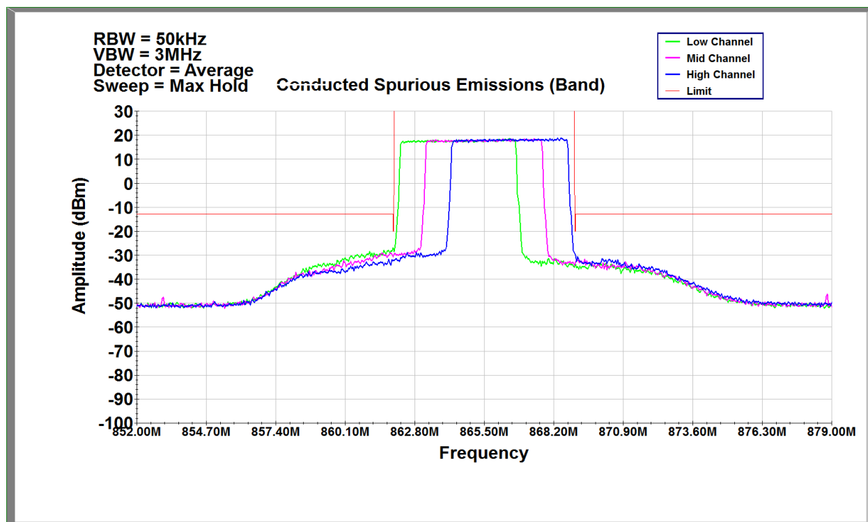
Band 26, Band Edge, 5MHz Bandwidth Setting, QPSK (part 90.691 limit shown)
