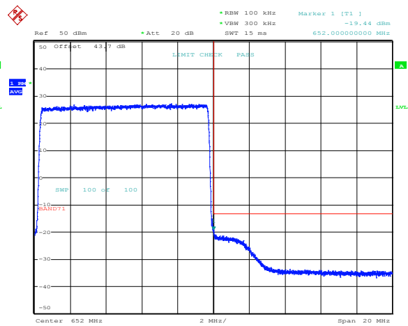
Band 71, Band Edge, 10MHz Bandwidth Setting, 64QAM
