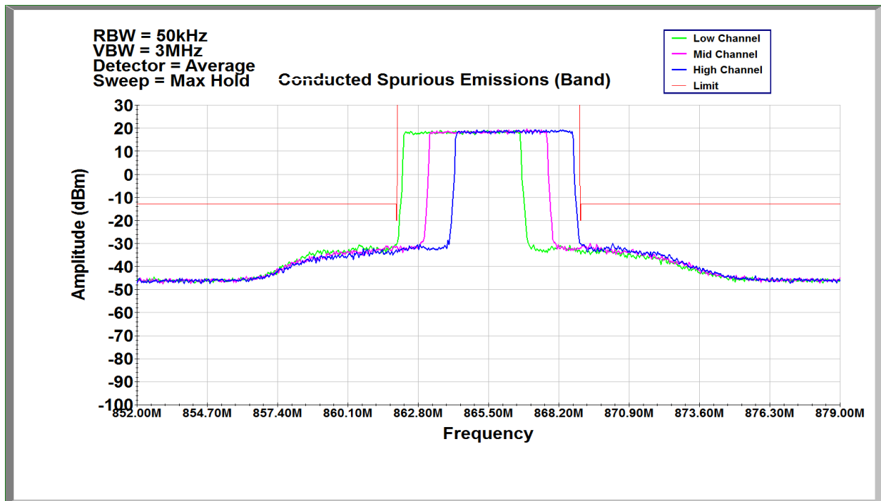
Band 26, Band Edge, 5MHz Bandwidth Setting, 256QAM (part 90.691 limit shown)
