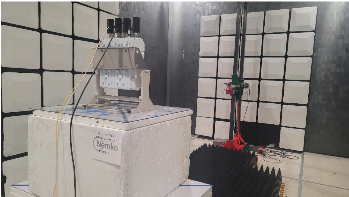
Figure 4 - Radiated emissions above 1 GHz (1 – 18 GHz), rear view.
