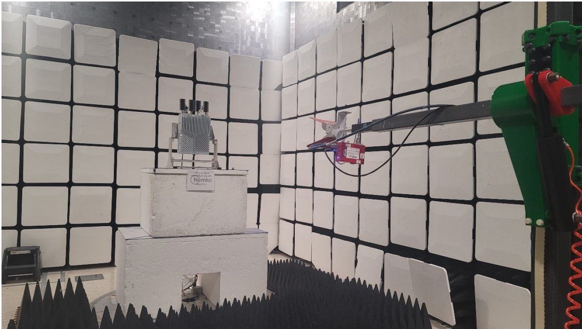
Figure 3 - Radiated emissions above 1 GHz (1 – 18 GHz), front view.
