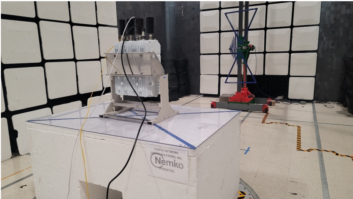
Figure 2 - Radiated emissions below 1 GHz (0.03 – 1 GHz), rear view.
