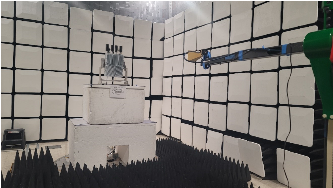
Figure 5 - Radiated emissions above 1 GHz (18 – 26 GHz), front view.
