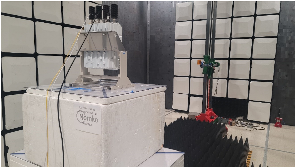
Figure 6 - Radiated emissions above 1 GHz (18 – 26 GHz), rear view.
