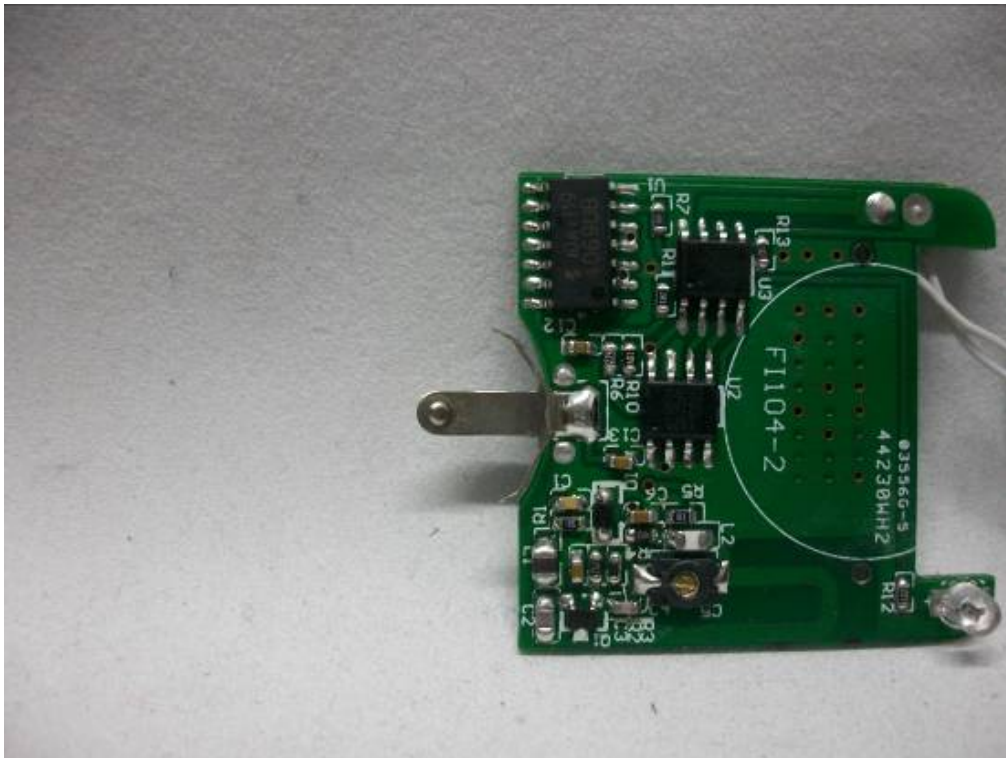
FRONT OF PCB1 VIEW
