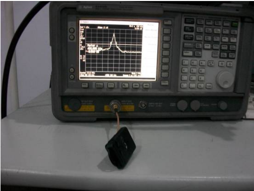
Spurious Emission Test Setup
