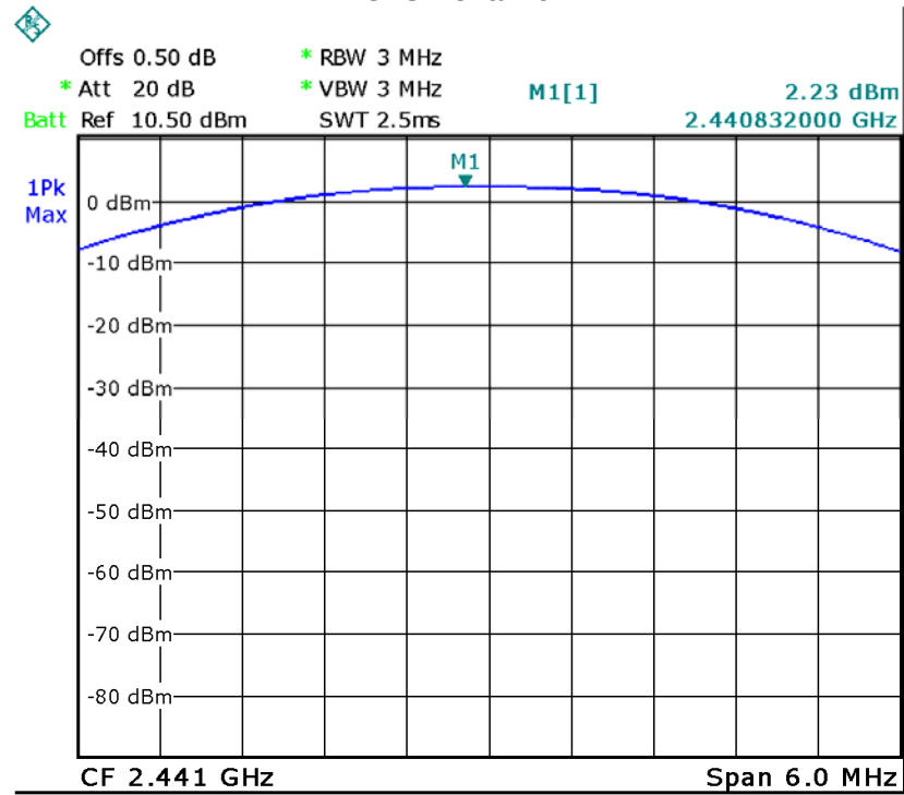
GFSK Channel
