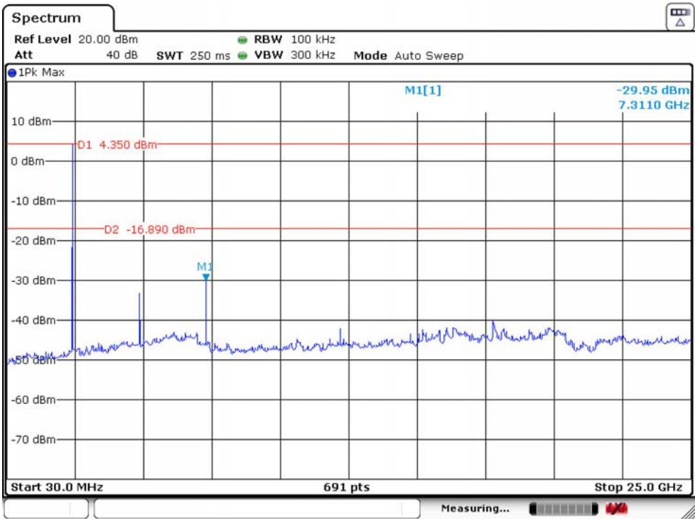
GFSK 2440 MHz
